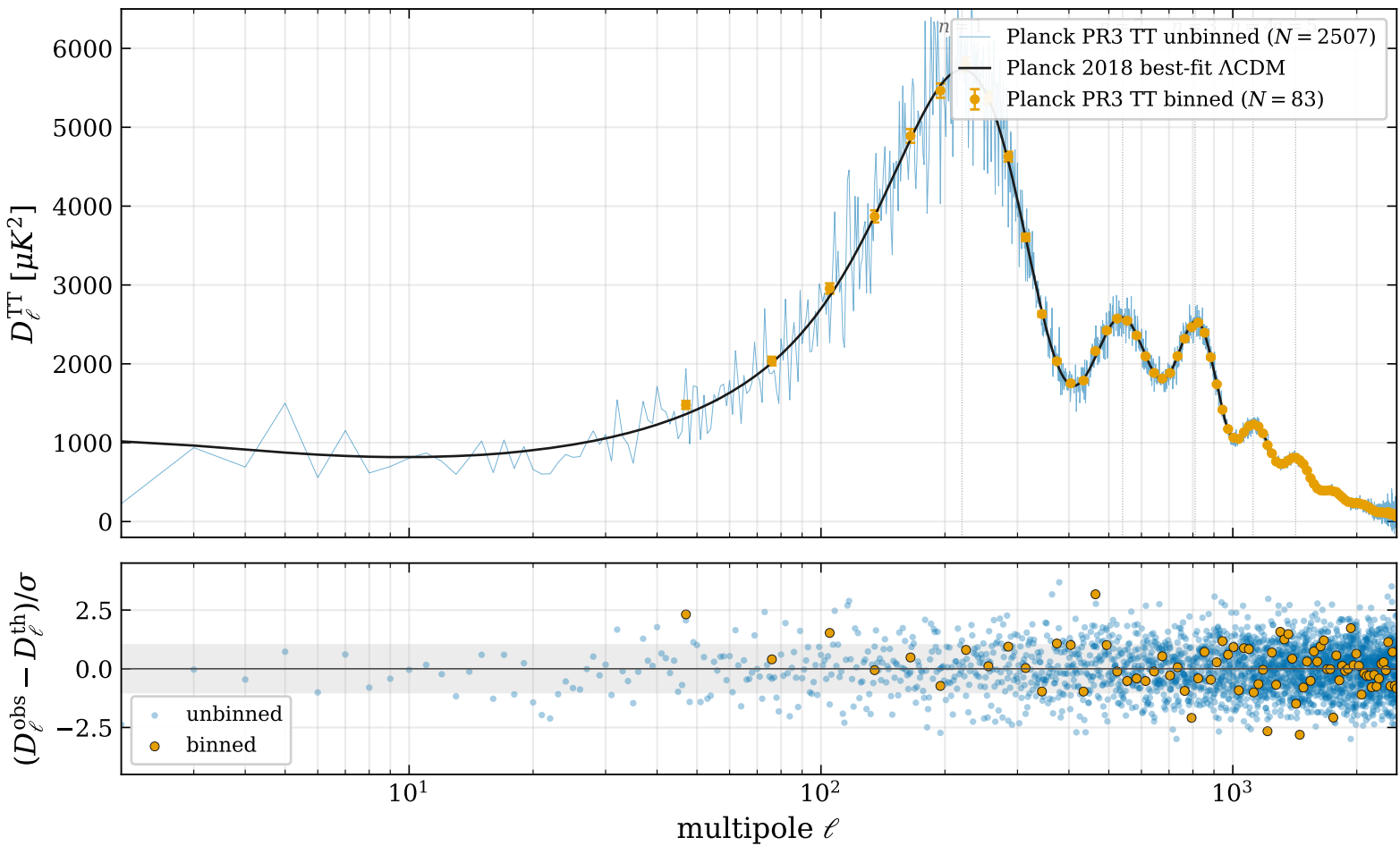
Planck PR3 TT — ell-by-ell unbinned points + binned summary ( \ell \in [2, 2500] )
