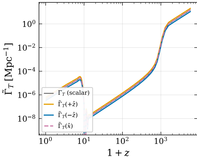
Thomson rate anisotropy at \beta = 0.30
