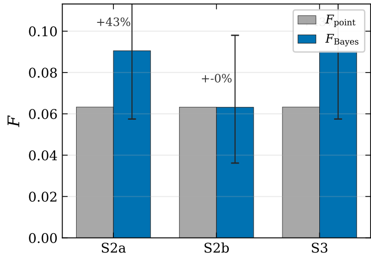
posterior-mean vs point estimate
