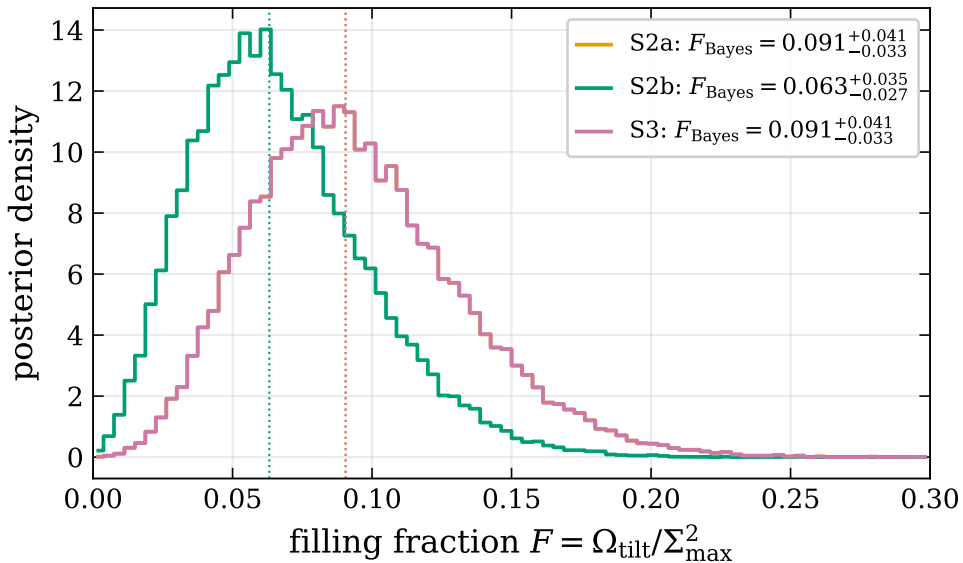
Monte Carlo posterior on F_{\text{Bayes}} (htt \times tsc)
