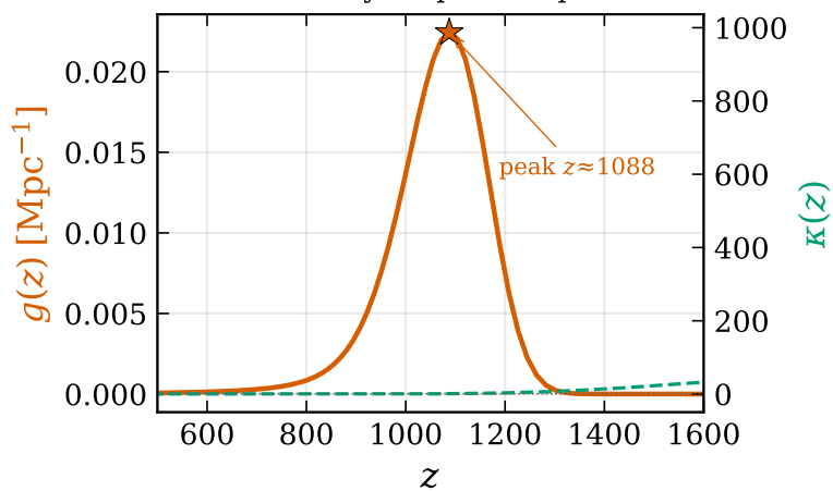
Visibility + optical depth
