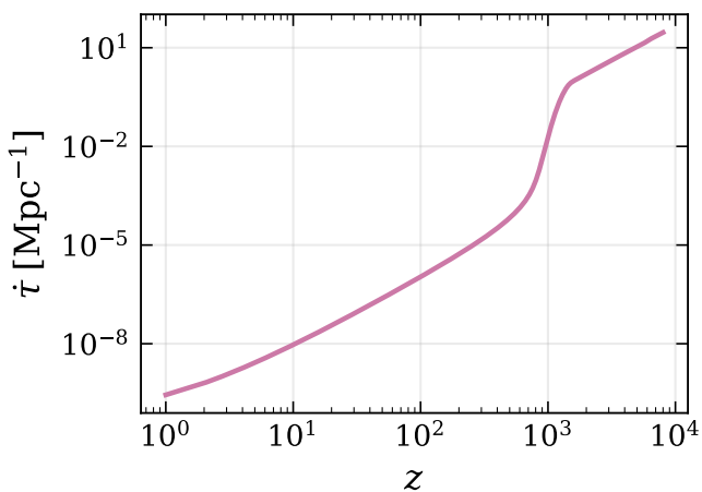
Thomson rate \dot{\tau}(z)
