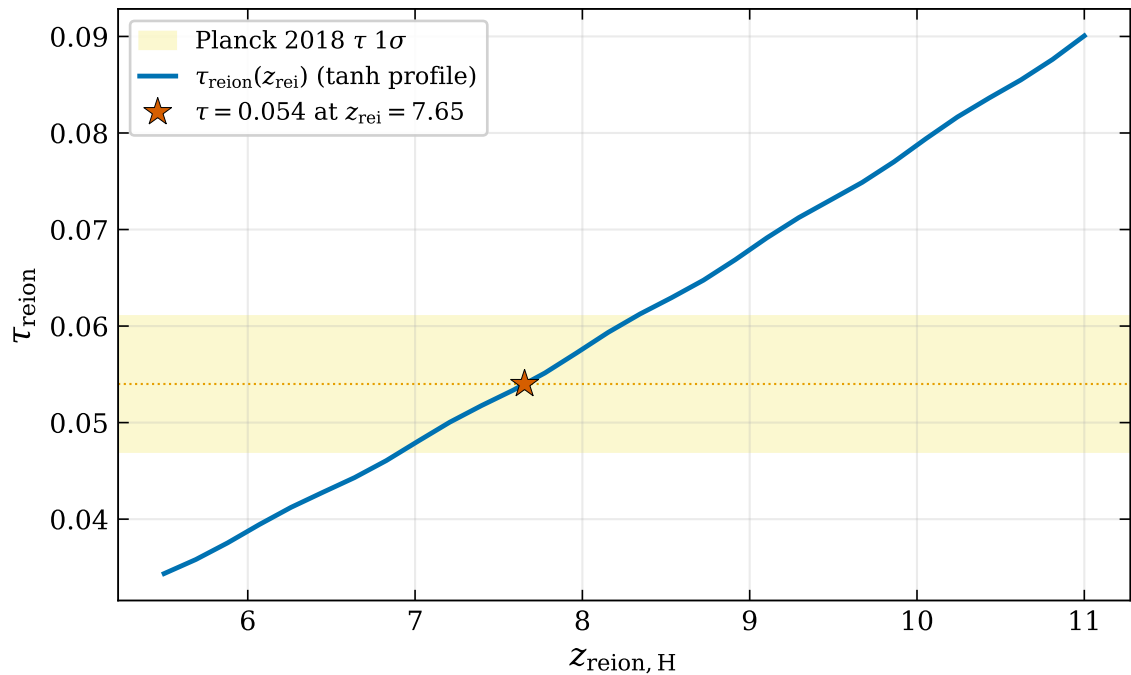
Reionization optical depth vs midpoint redshift
