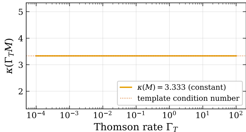
TCA matrix condition number
