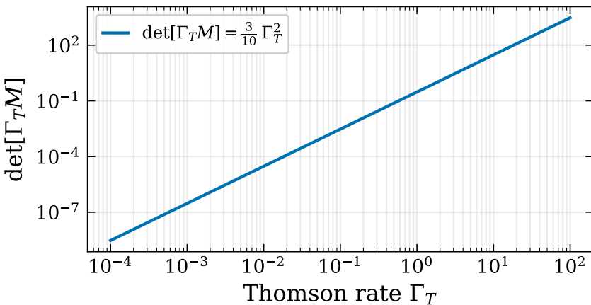
TCA matrix determinant
