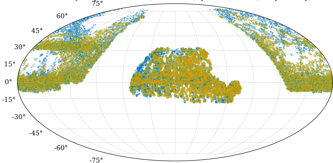
DESI Y1 sky footprint — 3 tracers, NGC+SGC (equatorial, max 15,000 points/cap)
