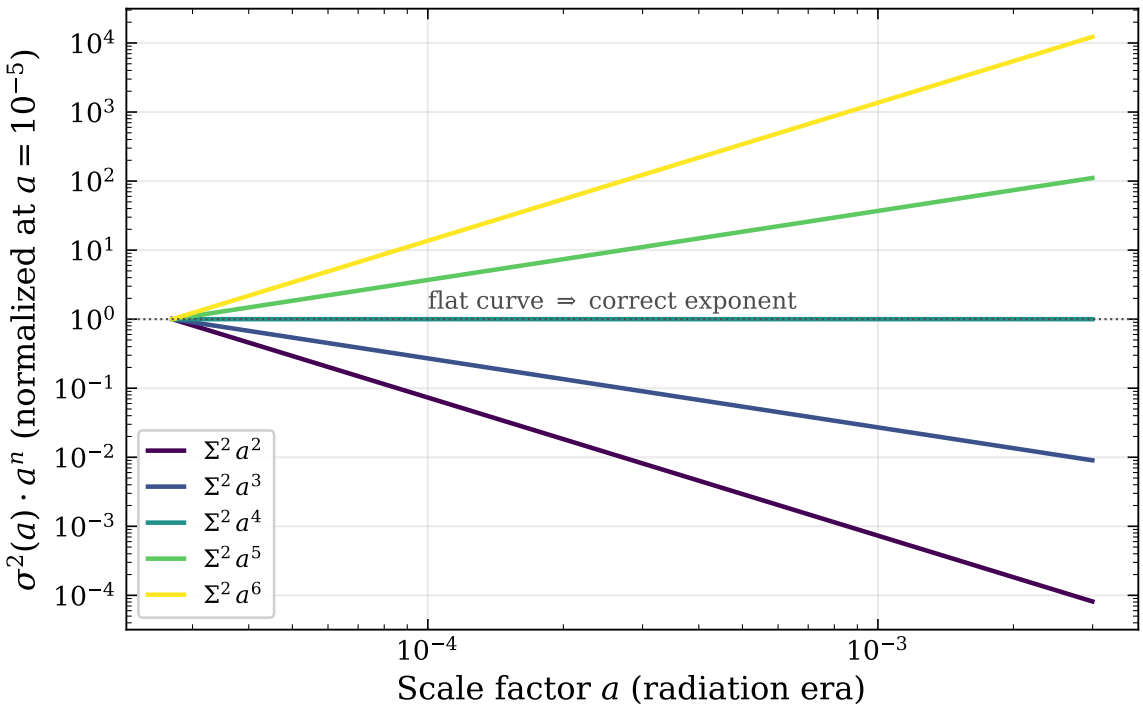
Power-law decay diagnostic: conformal shear \sigma_{ab}\sigma^{ab} \propto a^{-4}
