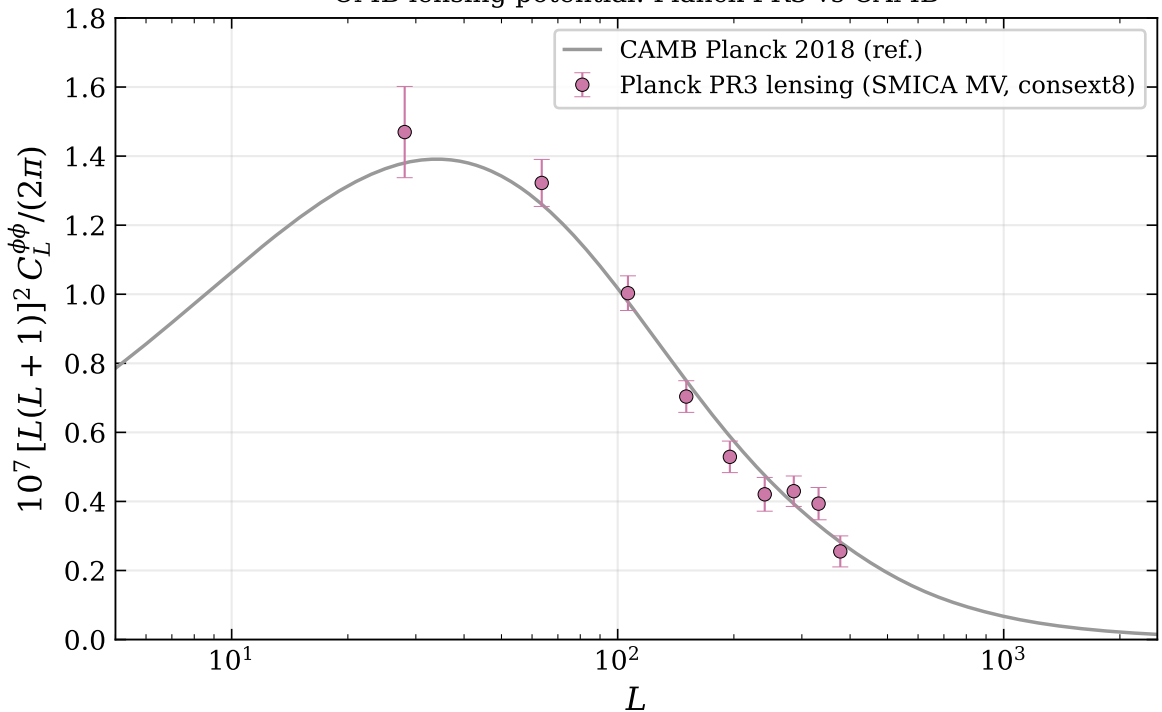
CMB lensing potential: Planck PR3 vs CAMB
