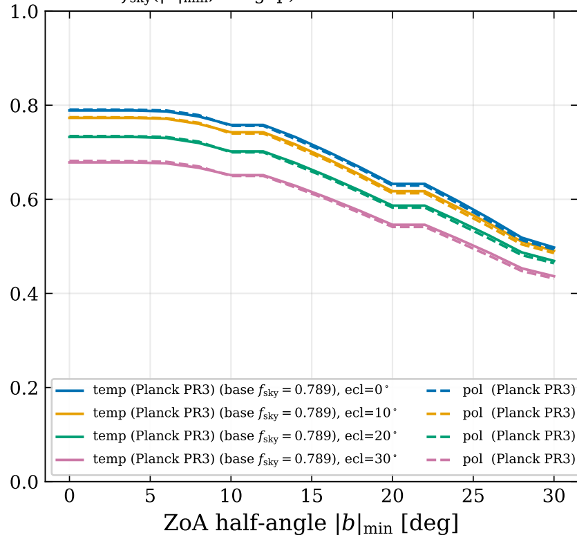
f_{\text{sky}}(|b|_{\min}, \text{ecl gap}) on real Planck masks
