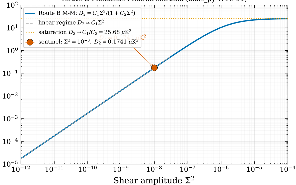
Route B Michaelis-Menten sentinel (bass_py W10-01)
