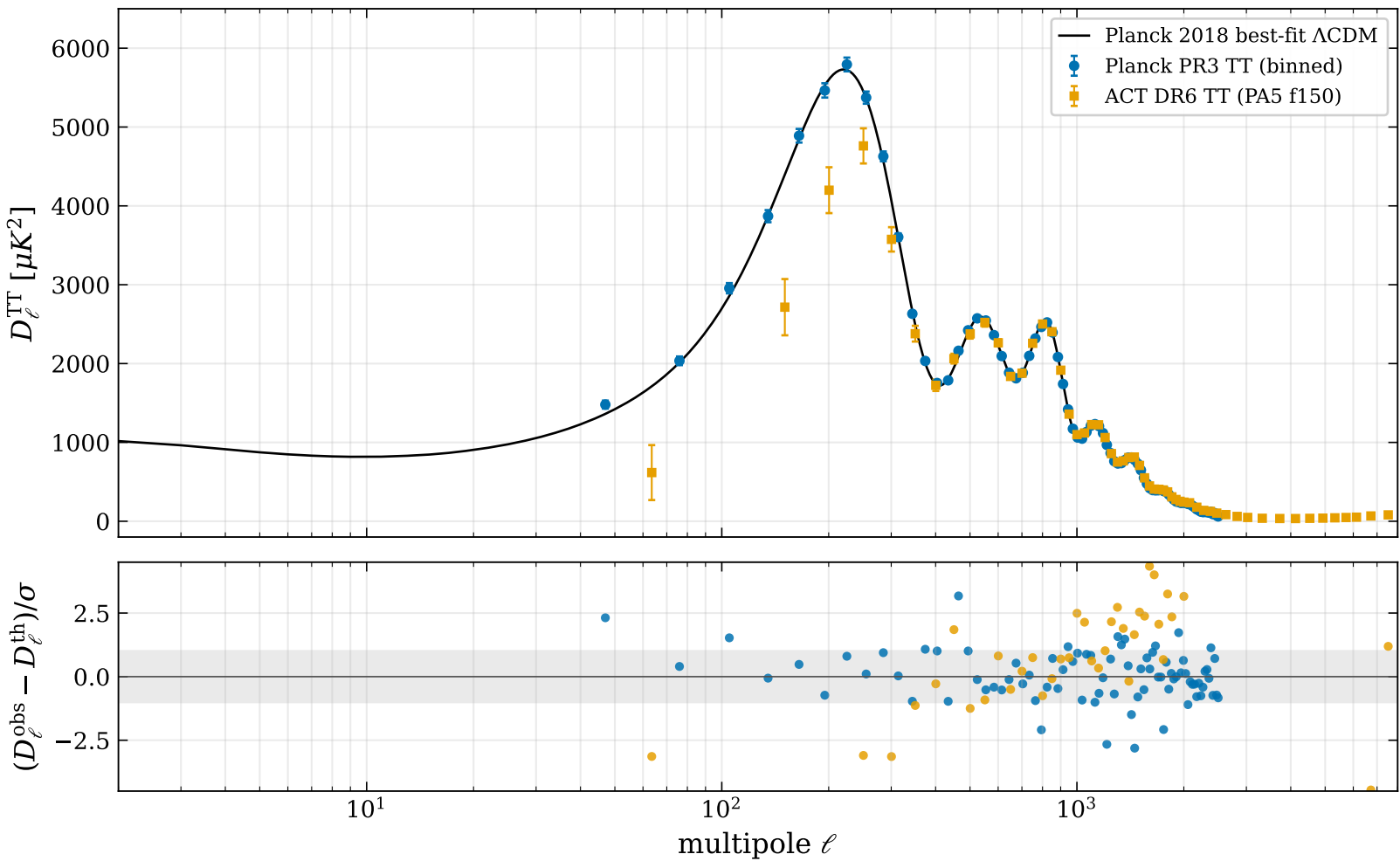
Multi-experiment CMB TT — Planck PR3 \cup ACT DR6 vs best-fit \Lambda CDM
