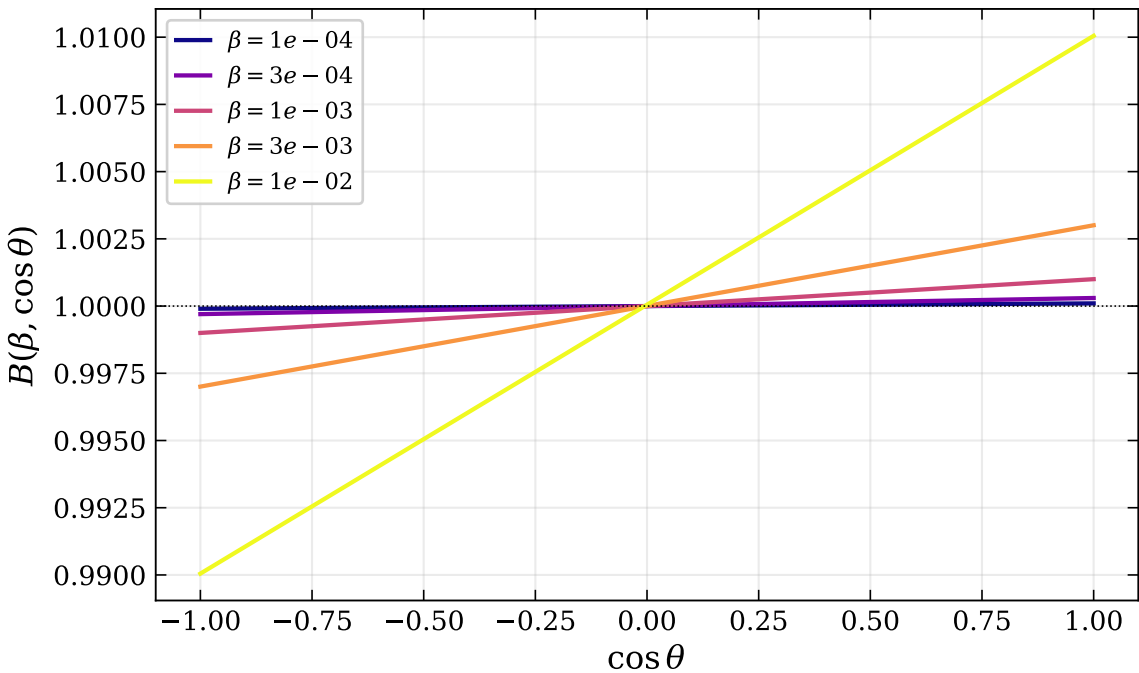
Forward/backward tilt asymmetry
