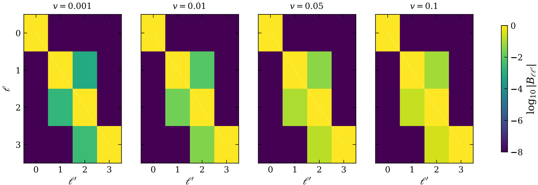
Prop 5 linearised boost mixing matrix B_{\ell\ell'}(\nu) — tsc. charts. boost_coefficients
