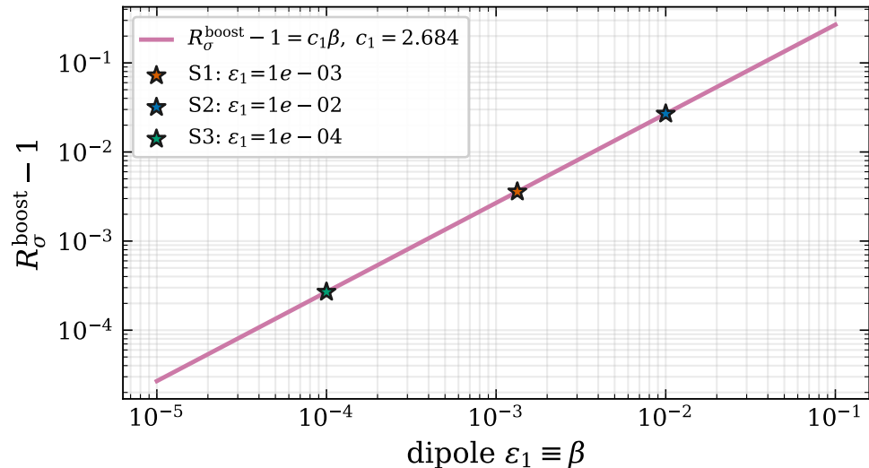
Layer-1 shear-bound correction R_\sigma^{\text{boost}}
