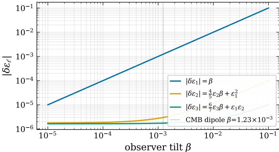
O(\beta) Doppler kernel ( \varepsilon fixed at VN-04 S1 triple)
