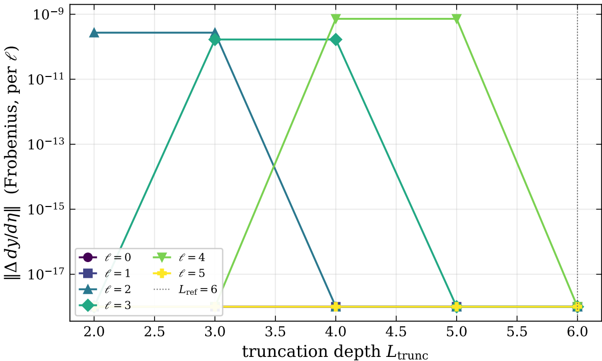
PSTF hierarchy closure convergence (Bianchi I, \sigma_+ \approx 3 \times 10^{-4} )
