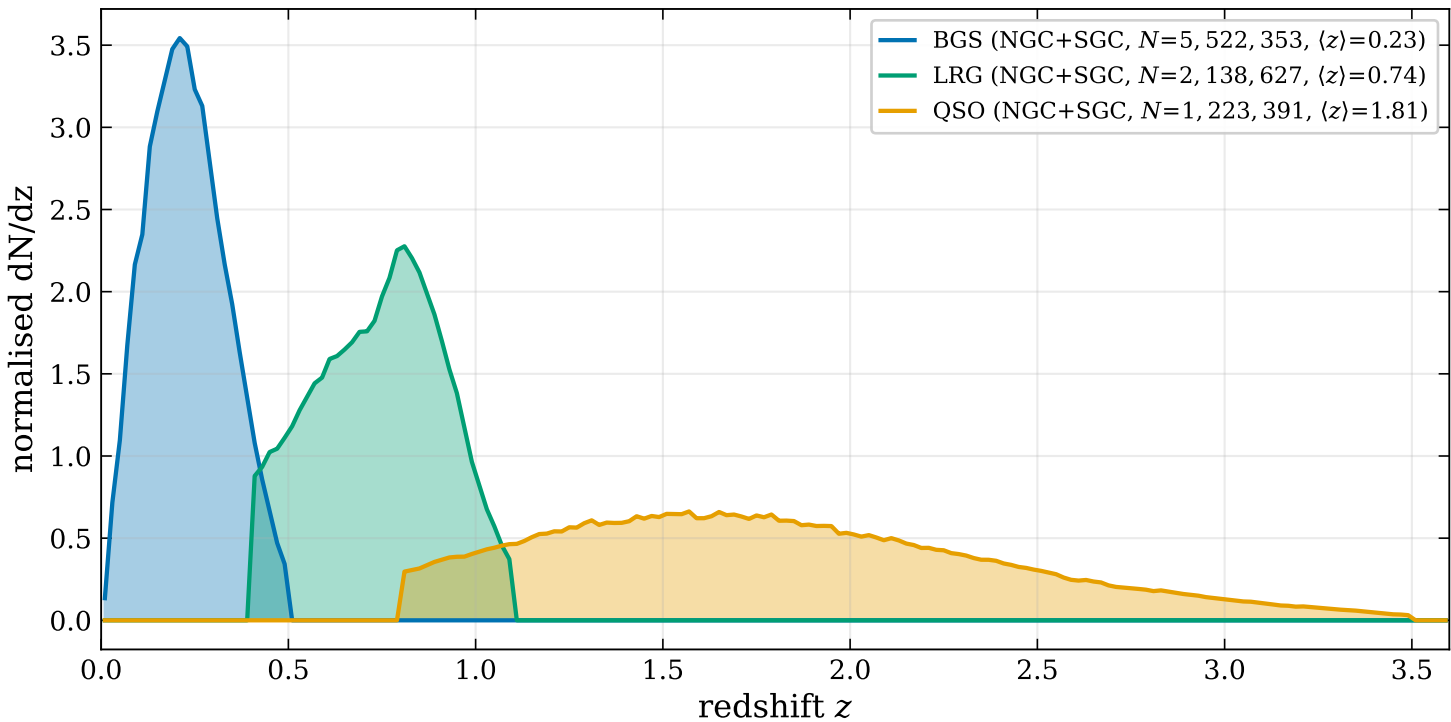
DESI Y1 weighted redshift distributions — 3 tracers, 8.88M galaxies
