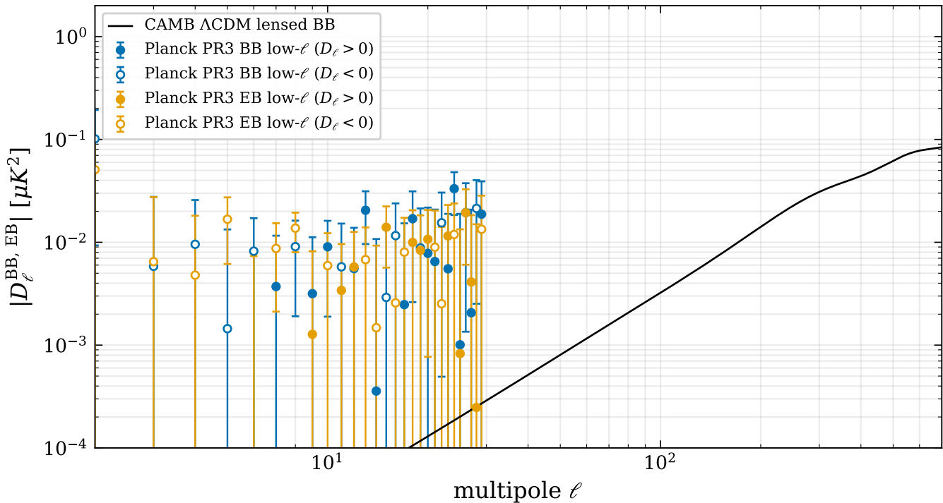
Planck PR3 low- \ell BB and EB polarization vs \Lambda CDM lensed-BB reference
