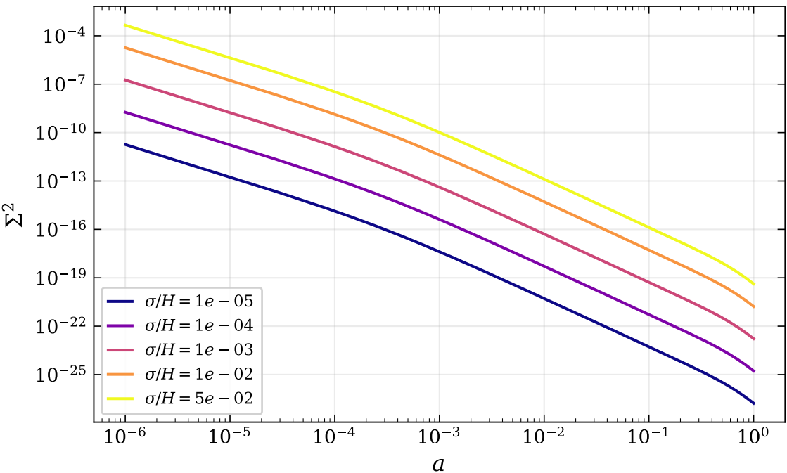
Bianchi I seed sweep
