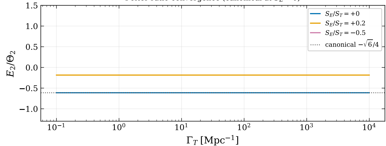
Polter ratio convergence (canonical at S_E = 0 )
