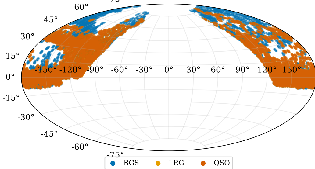
DESI Y1 NGC sky footprint (subsampled)
