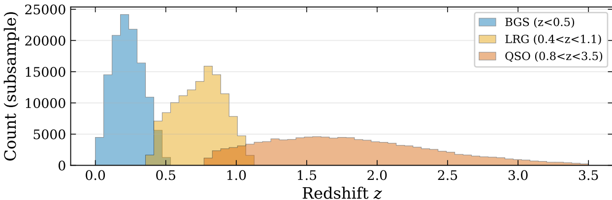
DESI Y1 NGC redshift distribution
