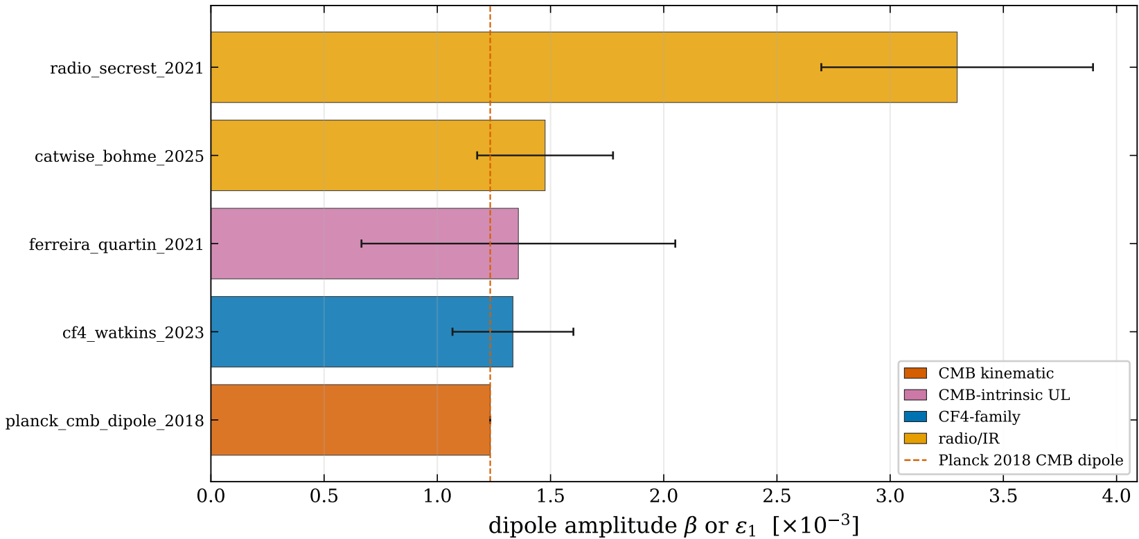
Cross-survey preferred-axis dipole amplitude compilation
