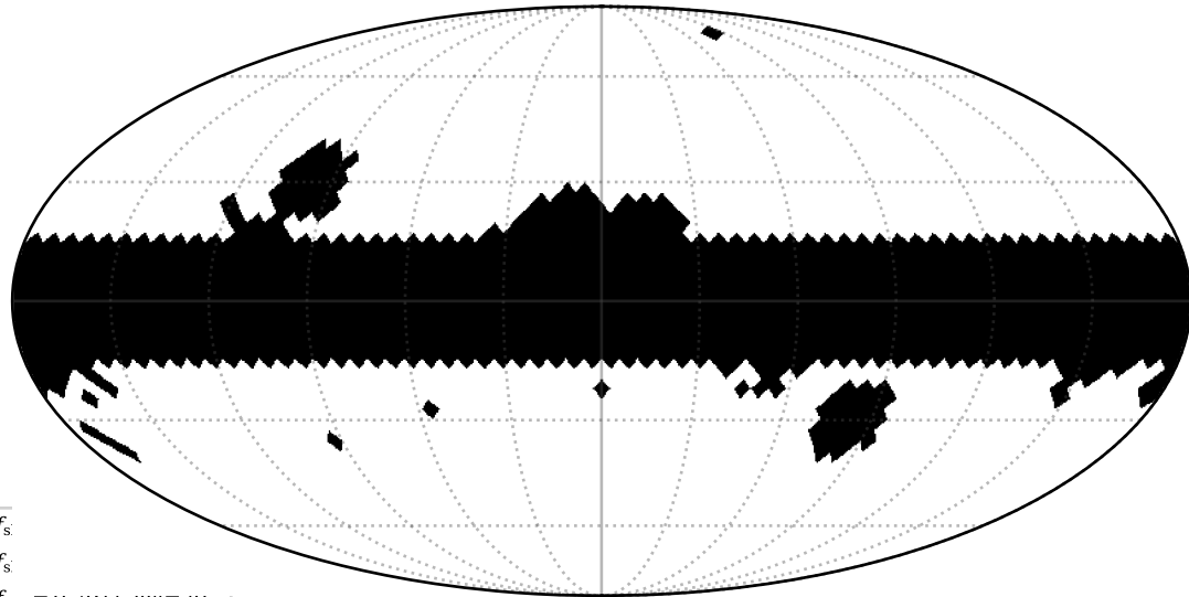
temp mask \cap (ZoA=15°, ecl=10°), f_{\text{sky}} = 0.686
