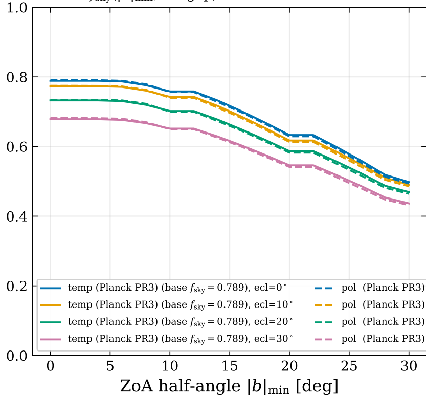
f_{\text{sky}}(|b|_{\text{min}}, \text{ecl gap}) on real Planck masks
