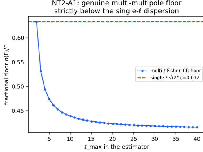
Figure 14: NT2-A1 multi-multipole Fisher floor (fractional dispersion \sigma(F)/F versus the estimator \ell_{\max} ), conditional on the registered shear-response profile and below the single- \ell dispersion under that response. Diagnostic-only; synthetic.
