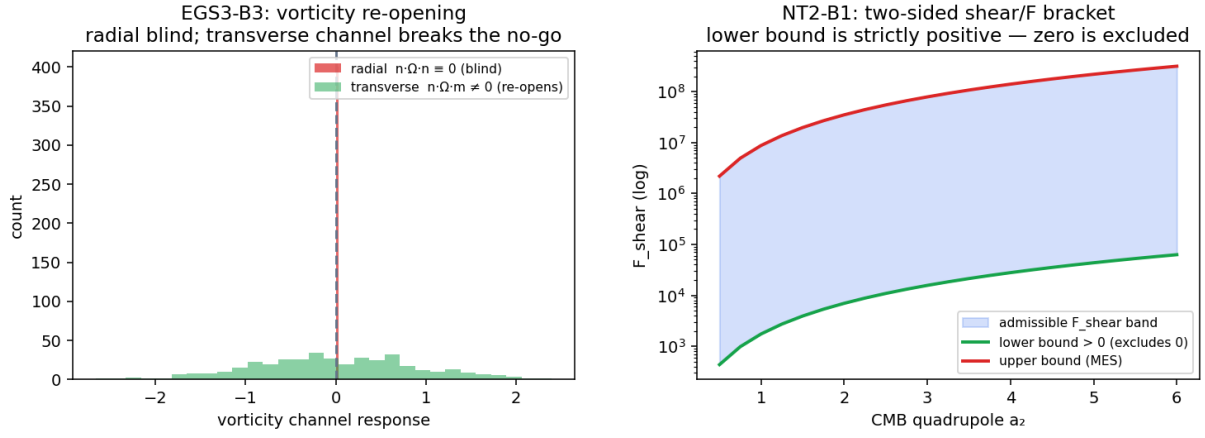
Figure 16: Axis B. Left: EGS3-B3, radial peculiar velocities are vorticity-blind ( n^a \Omega_{ab} n^b \equiv 0 ) while the transverse channel re-opens the sector. Right: NT2-B1, the two-sided shear/ F bracket; within the registered closure/H3 model the lower bound is strictly positive so the closure-defined shear-filling is excluded from zero at fixed a_2 . Diagnostic-only; synthetic.
