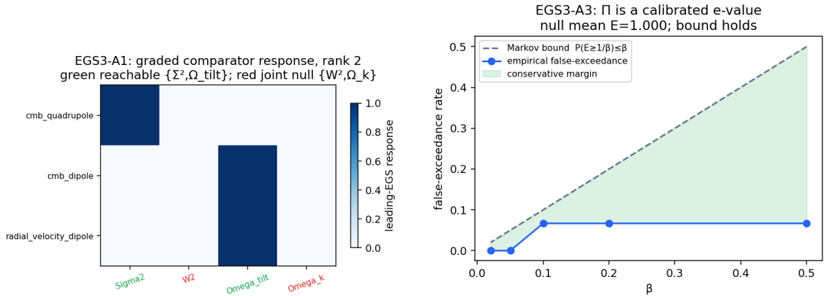
Figure 13: Axis A. Left: EGS3-A1 graded-comparator response, rank two within the registered leading-channel response map (green reachable; red the two-sector null— W_{\text{std}}^2 a genuine structural null, \Omega_{k,\text{aniso}} a leading-order no-channel). Right: EGS3-A3, \Pi as a calibrated e-value with a Markov false-exceedance bound under the GRF- \Lambda CDM null. Diagnostic-only; synthetic; no detection or family identification.
