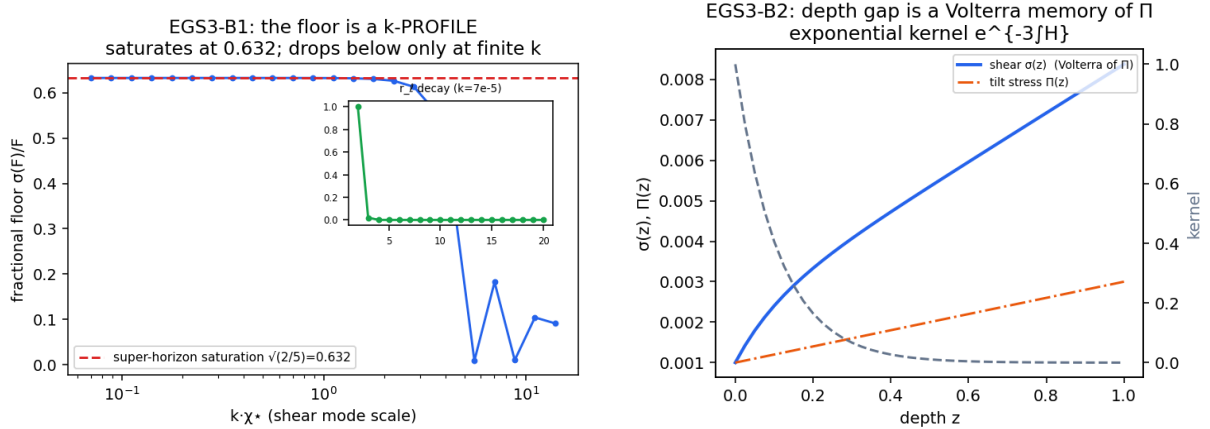
Figure 15: Axis B. Left: EGS3-B1, the floor is a single-mode, finite- k k -profile (sharpening NT2-A1 under the registered response). Right: EGS3-B2, the depth gap is a Volterra functional of the tilt anisotropic stress with kernel e^{-3\int H} . Diagnostic-only; synthetic.
