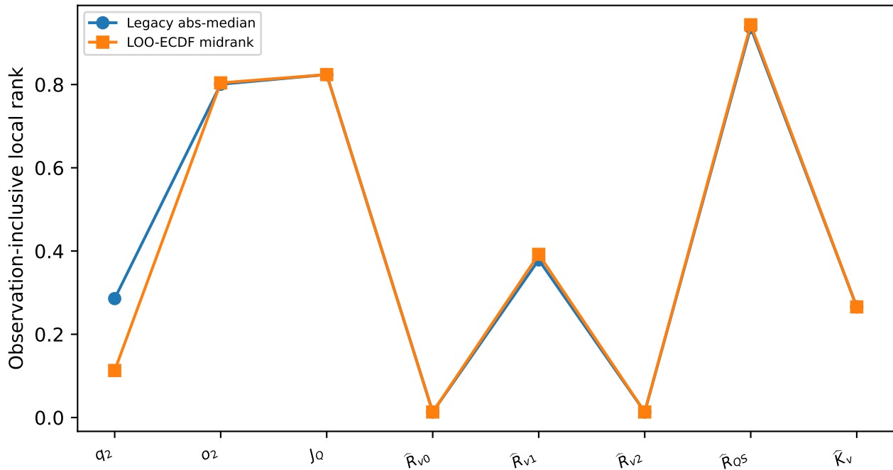
Observed frame-free irrep coordinates
