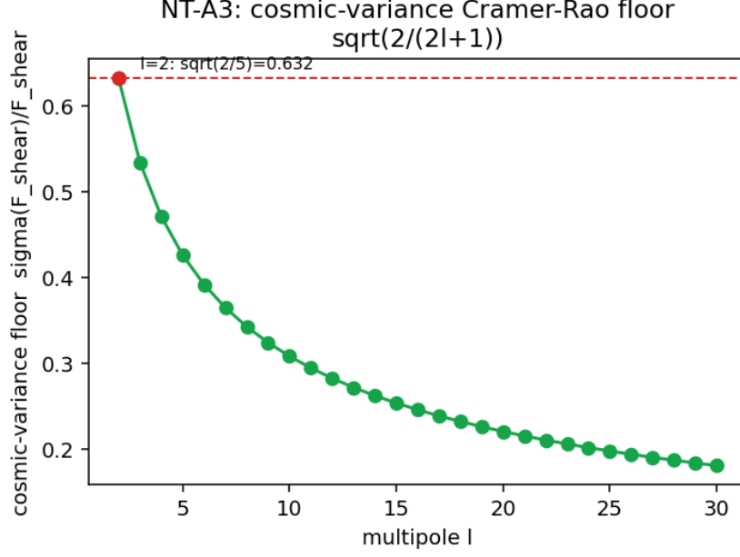
Figure 2: Theorem 2 (NT-A3): the single-sky fractional sampling dispersion \sqrt{2/(2\ell + 1)} of the standard full-sky F_{\text{shear}} estimator, equal to \sqrt{2/5} \approx 0.632 at the quadrupole (not a universal floor). Diagnostic-only; not a detection.
