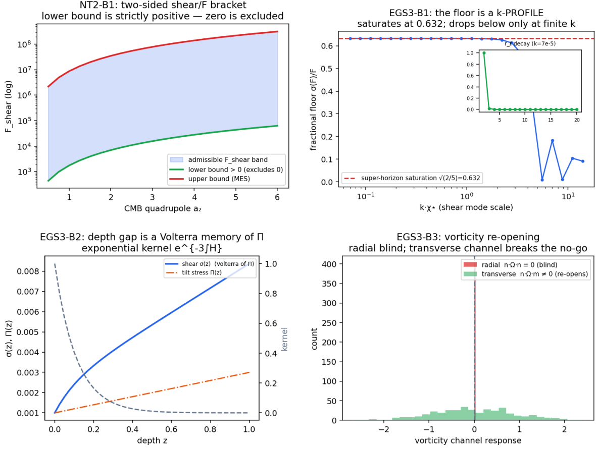
Figure 12: Carried set II. Top: two-sided reciprocal shear bracket (Proposition 4.19); registered transfer floor profile (Proposition 4.14). Bottom: Volterra depth memory (Proposition 3.15); transverse vorticity reopening (Proposition 3.13).
