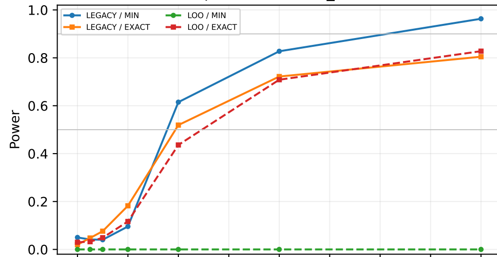
cmbonly999: MES_10
