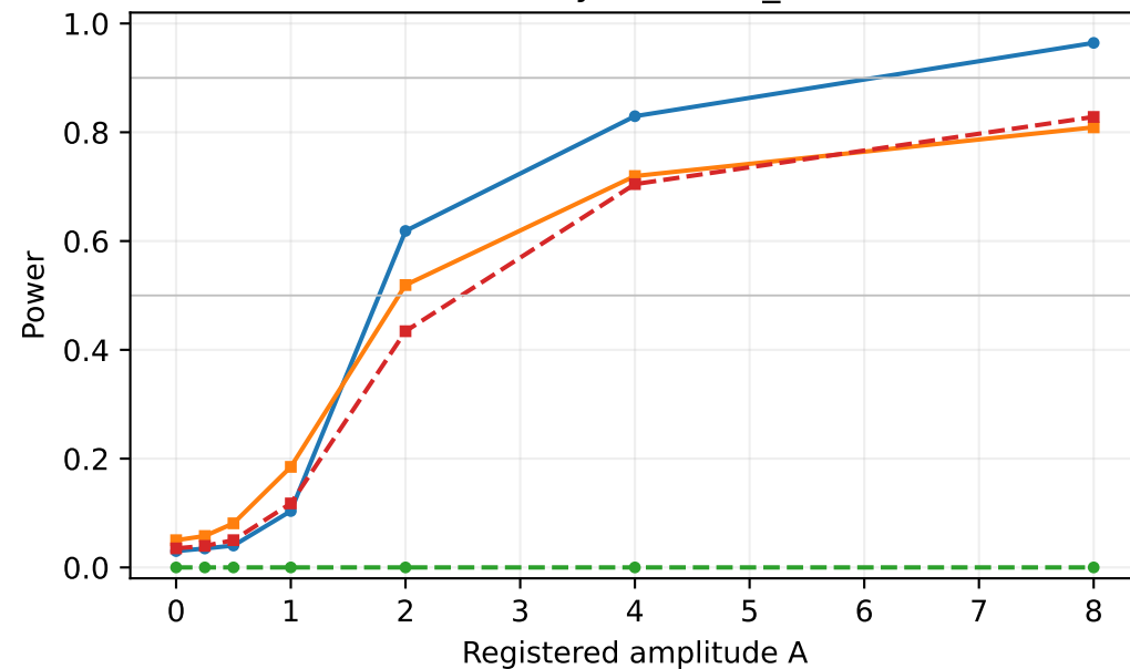
cmbonly999: MES_10
