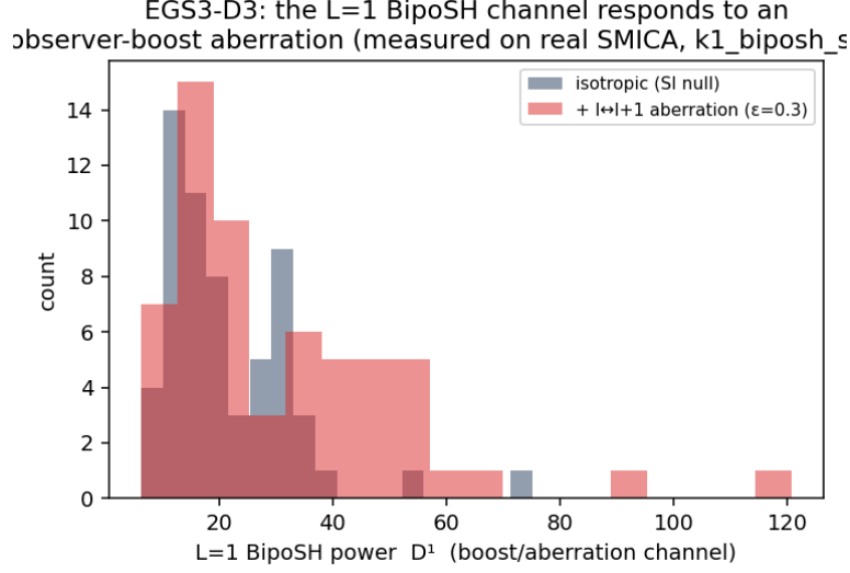
Figure 20: Axis D, the L=1 Bipolar-Spherical-Harmonic (BipoSH) channel. The rotationally-invariant L=1 power D^1 (the observer-boost/aberration \ell \leftrightarrow \ell+1 coupling) responds to an injected aberration, the mechanism underlying the real SMICA/Commander BipoSH measurement ( scripts/k1_biposh_smica.py ). Diagnostic-only SI descriptor; no family/geometry/native-solver claim.
