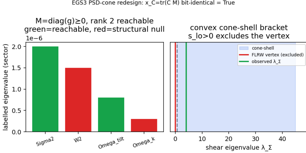
Figure 17: EGS3 PSD-cone redesign. Left: M = \text{diag}(g) \succeq 0 , rank-two reachable eigen-directions (green) versus the structural null (red). Right: the convex cone-shell \{M \succeq 0 : s_{\text{lo}} < \lambda_\Sigma < s_{\text{hi}}\} excluding the FLRW vertex. Representation only, gated behind the additive upgrade; diagnostic-only.
