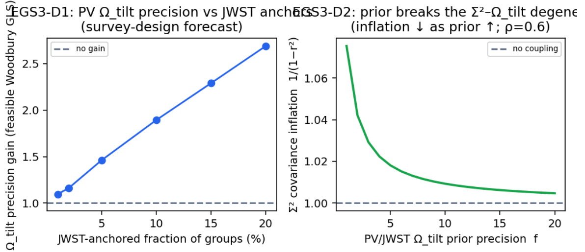
Figure 19: Axis D, BASS-Extended joint PV+CMB forecast. Left: the \Omega_{\text{tilt}} precision gain from a JWST-anchored distance prior versus the anchored fraction of groups (feasible correlated-covariance Woodbury GLS on real CF4; a survey-design forecast). Right: the \Sigma_{\text{std}}^2 covariance inflation 1/(1-r^2) falls as the PV/JWST \Omega_{\text{tilt}} prior precision f rises — the prior breaks the \Sigma_{\text{std}}^2 - \Omega_{\text{tilt}} degeneracy. Forecast; \Sigma_{\text{std}}^2 stays partial; the theory-g CMB likelihood is fail-closed.
