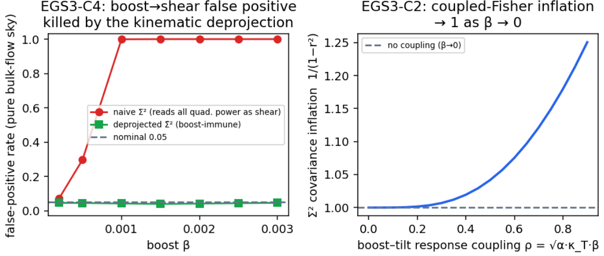
Figure 18: Axis C, kinematic deprojection of the observer-boost quadrupole. Left: on a pure-bulk-flow sky the naive \Sigma_{\text{std}}^2 false-positive rate (red) rises to nearly one as the boost \beta grows, while the deprojected \widetilde{\Sigma}_{\text{std}}^2 (green) stays at the nominal level. Right: the coupled-Fisher \Sigma_{\text{std}}^2 covariance inflation 1/(1-r^2) versus the boost-tilt response coupling \rho = \sqrt{\alpha} \kappa_T \beta , returning to unity as \beta \rightarrow 0 . Deterministic moment-level synthetic mechanics; diagnostic-only; no map, no native low- \ell solver, no real data; \Sigma_{\text{std}}^2 stays partial.
