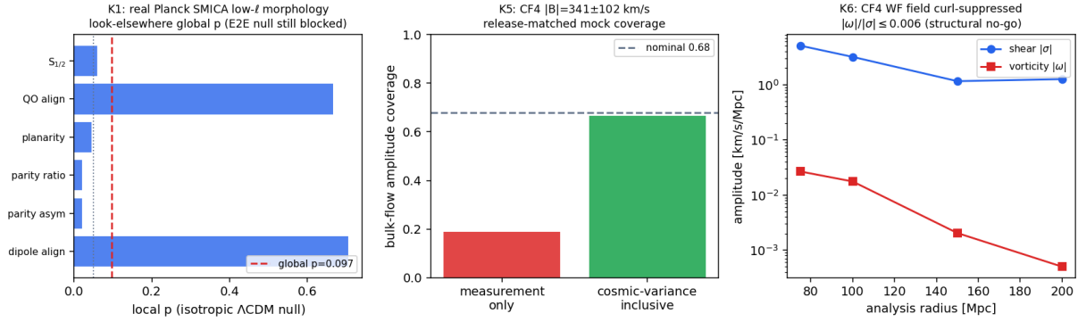
Figure 21: Real-data blocker discharges. K1 : per-statistic local and look-elsewhere global p of the real Planck SMICA low- \ell morphology under an isotropic \Lambda CDM null (the E2E-systematics null stays blocked). K5 : CF4 bulk-flow amplitude coverage — measurement-only under-covers, the cosmic-variance-inclusive coverage is nominal. K6 : the CF4 WF velocity field has vorticity \ll shear at every radius (curl-suppressed reconstruction; structural no-go). Diagnostic-only; model-independent.
