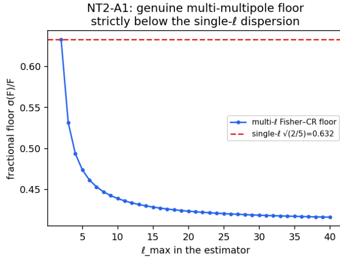
Figure 14: NT2-A1 multi-multipole Fisher floor (fractional dispersion \sigma(F)/F versus the estimator \ell_{\text{max}} ), conditional on the registered shear-response profile and below the single- \ell dispersion under that response. Diagnostic-only; synthetic.
