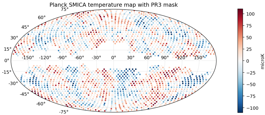
Figure 17: Planck SMICA nsid16 temperature pixels displayed under the PR3 temperature mask.
