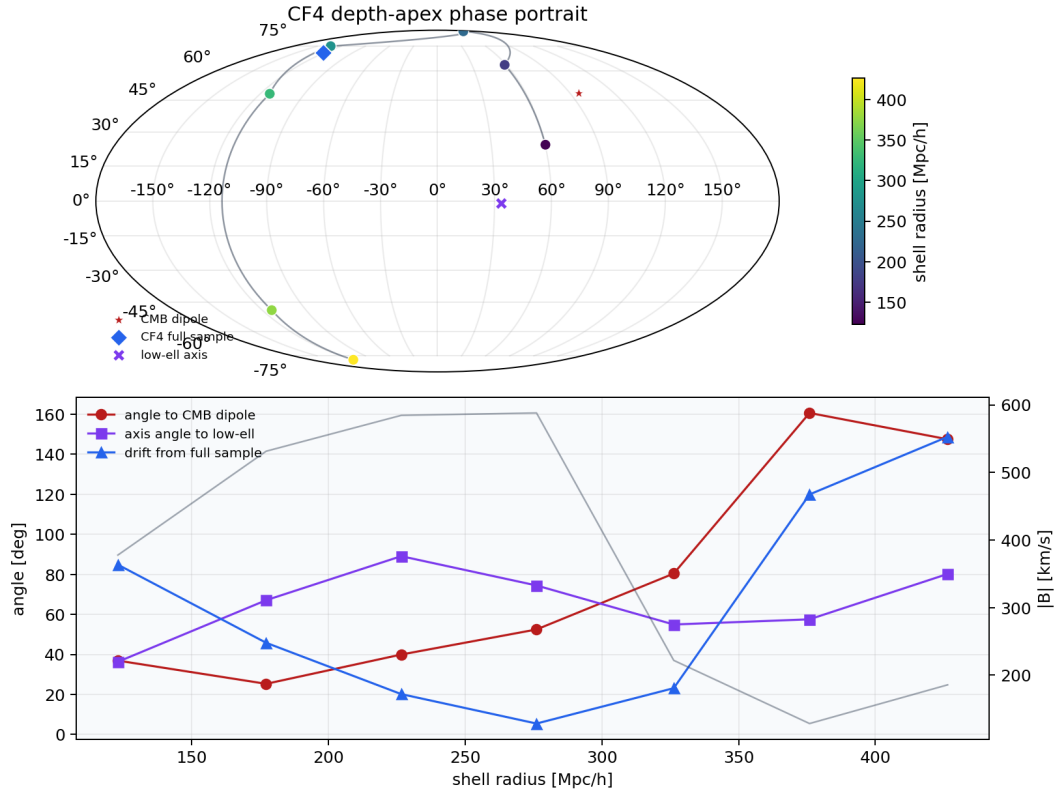
Figure 30: CF4++ reconstruction-functional shell-apex track with reference axes; method/systematics only while C1-K5-MV-F1 remains OPEN.
