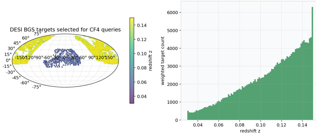
Figure 24: DESI BGS targets selected for CF4 queries, shown by sky position and redshift.
