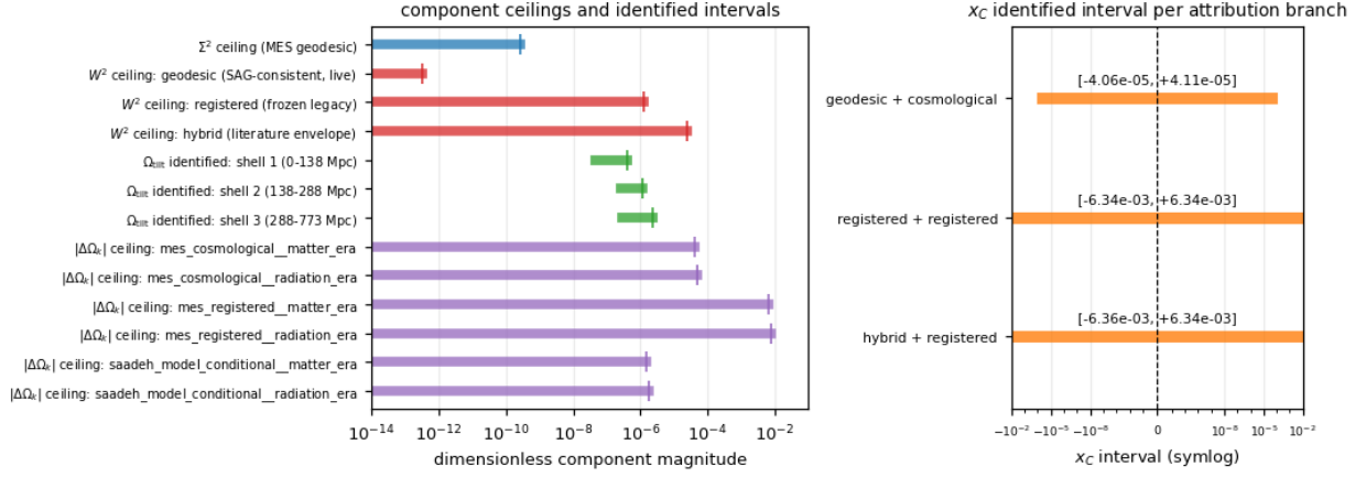
Figure 1: Assembled identified region for g and the induced x_C intervals per attribution branch (Section 5).
