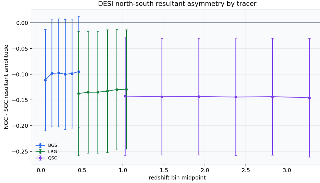
Figure 26: DESI NGC-minus-SGC resultant-amplitude differences as a function of tracer and redshift.
