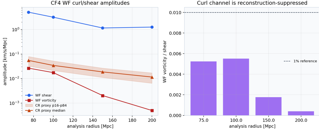
Figure 20: CF4 Wiener-filter velocity-field curl/shear diagnostic showing reconstruction-conditioned curl suppression.
