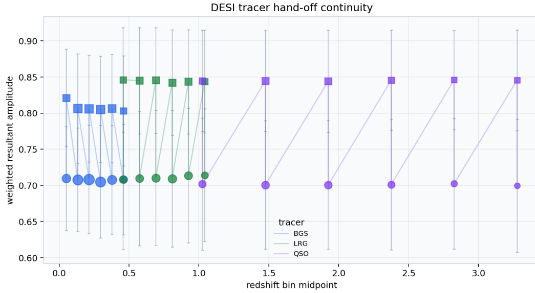
Figure 27: DESI tracer redshift hand-off shown with occupancy-scaled markers and jackknife uncertainty.
