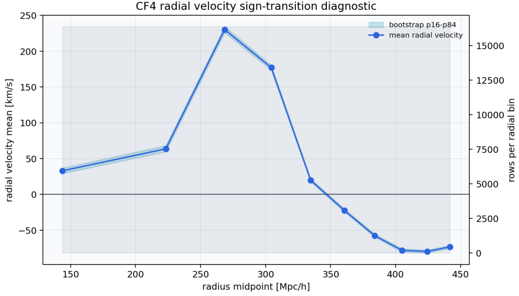
Figure 28: CF4 radial-shell mean velocity with bootstrap p16-p84 band and bin occupancy.
