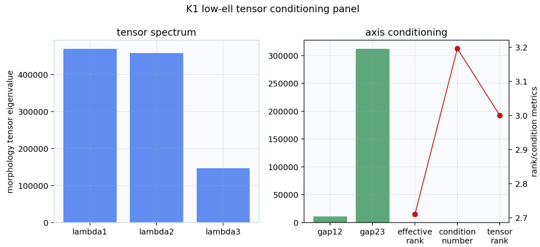
Figure 33: K1 low-ell morphology tensor eigenvalues, eigenvalue gaps, and conditioning metrics.
