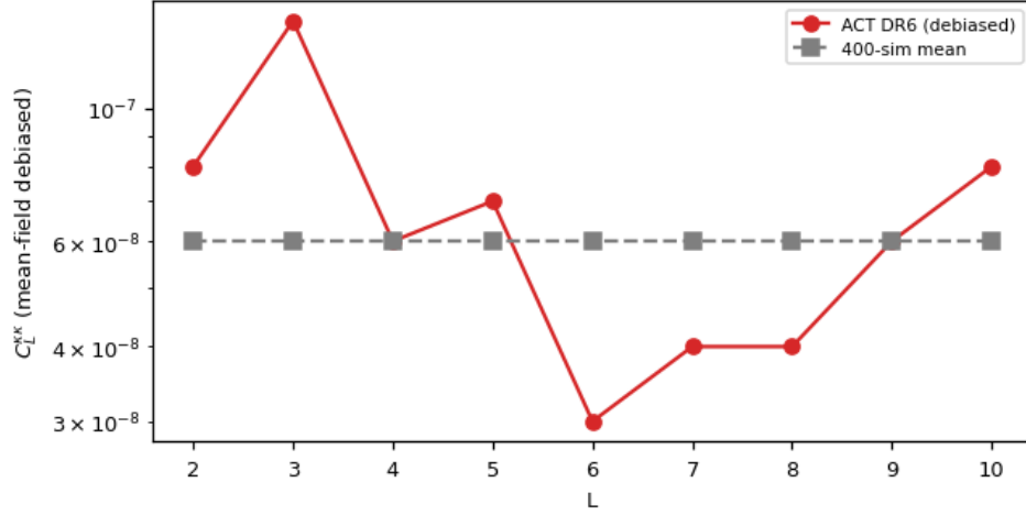
low-L band p = 0.35 ; 95% UL on excess band power 3.28e-06 ; in-band modulation rank 102/401
