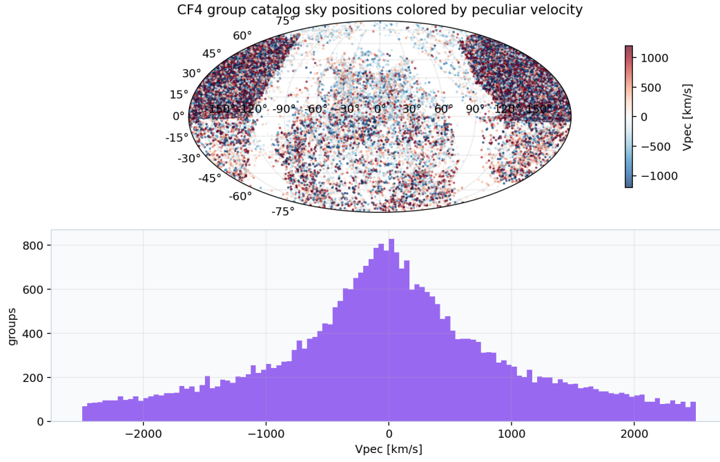
Figure 18: Cosmicflows-4 group sky positions colored by catalog peculiar velocity, with the velocity distribution below.
