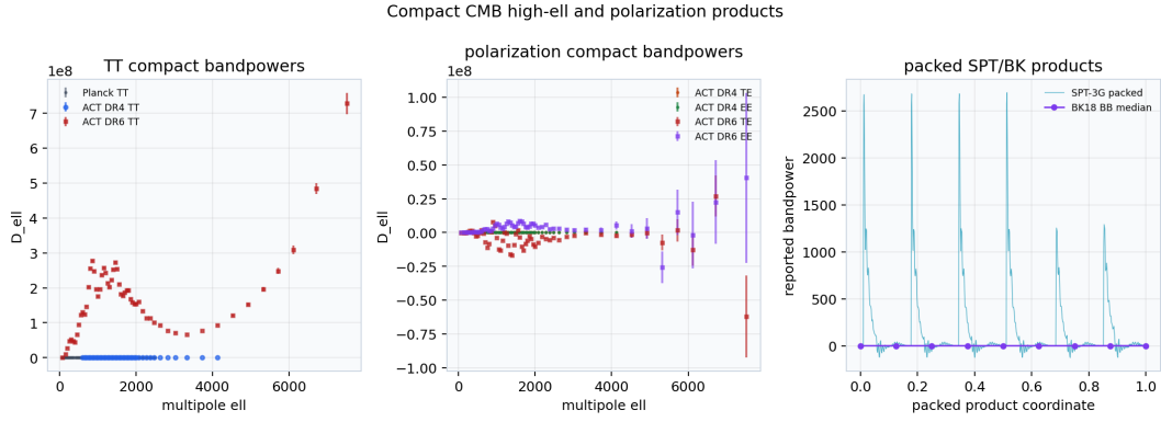
Figure 21: Compact Planck, ACT, SPT-3G, and BICEP/Keck CMB bandpower products, with ACT DR6 included when locally extracted.
