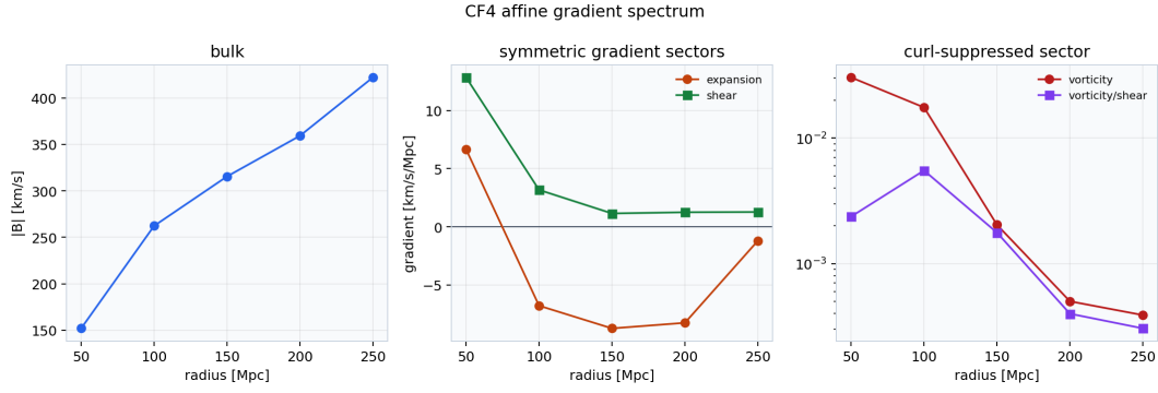
Figure 32: CF4++ affine reconstruction functionals versus radius; estimator/systematics only while C1-K5-MV-F1 remains OPEN.
