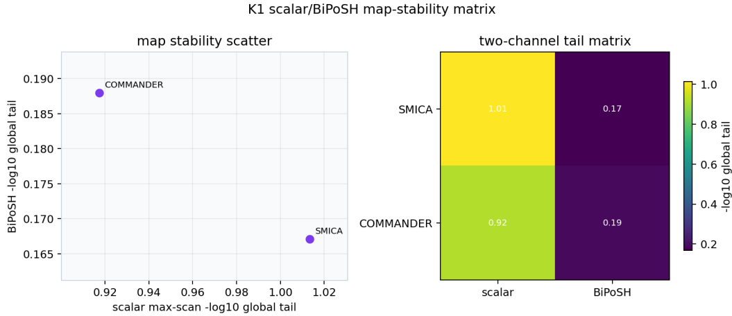
Figure 35: K1 scalar and BiPoSH two-channel global-tail comparison across map products.
