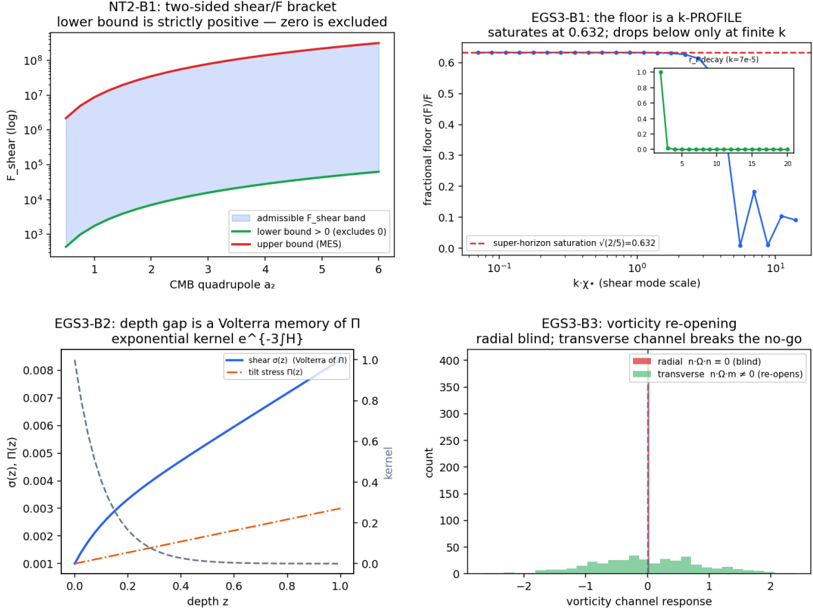
Figure 12: Carried set II. Top: two-sided reciprocal shear bracket (Proposition 4.20); registered transfer floor profile (Proposition 4.14). Bottom: Volterra depth memory (Proposition 3.15); transverse vorticity reopening (Proposition 3.13).
