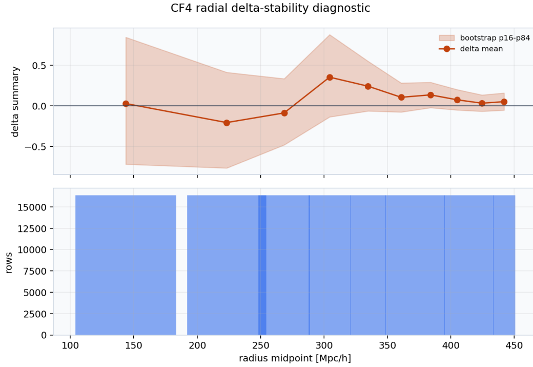
Figure 29: CF4 radial-shell delta summary with bootstrap band and row counts.
