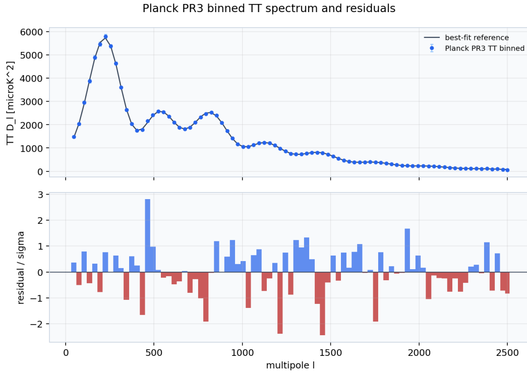
Figure 16: Planck PR3 binned TT spectrum with bundled best-fit reference and residuals.
