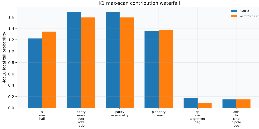
Figure 34: K1 local statistic contributions to the global max-scan for SMICA and Commander.
