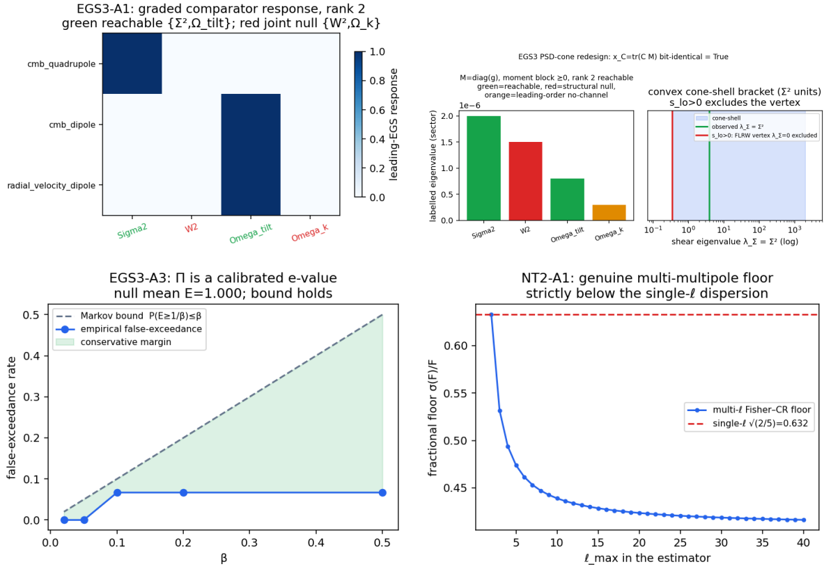
Figure 11: Carried set I. Top: rank-two response and joint null sector (Theorem 3.3); cone representation (Proposition 4.16). Bottom: exceedance/e-value calibration (Proposition 3.8); multi- \ell Fisher floor (Proposition 3.11).
