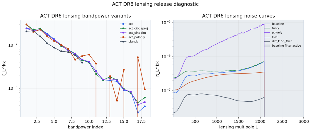
Figure 23: ACT DR6 lensing bandpower variants and release-provided noise curves; no ACT lensing likelihood or mock-calibrated inference is run.
