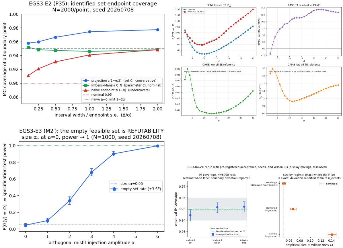
Figure 14: Carried set IV. Top: Imbens–Manski coverage certificate (Proposition 3.18); CAMB cross-check of the low- \ell spectrum lane supporting the transfer-floor cross-check (Proposition 4.14). Bottom: noncentral- \chi^2 refutability power (Proposition 3.16); estimated-covariance fingerprint coverage rerun (Proposition 3.18).
