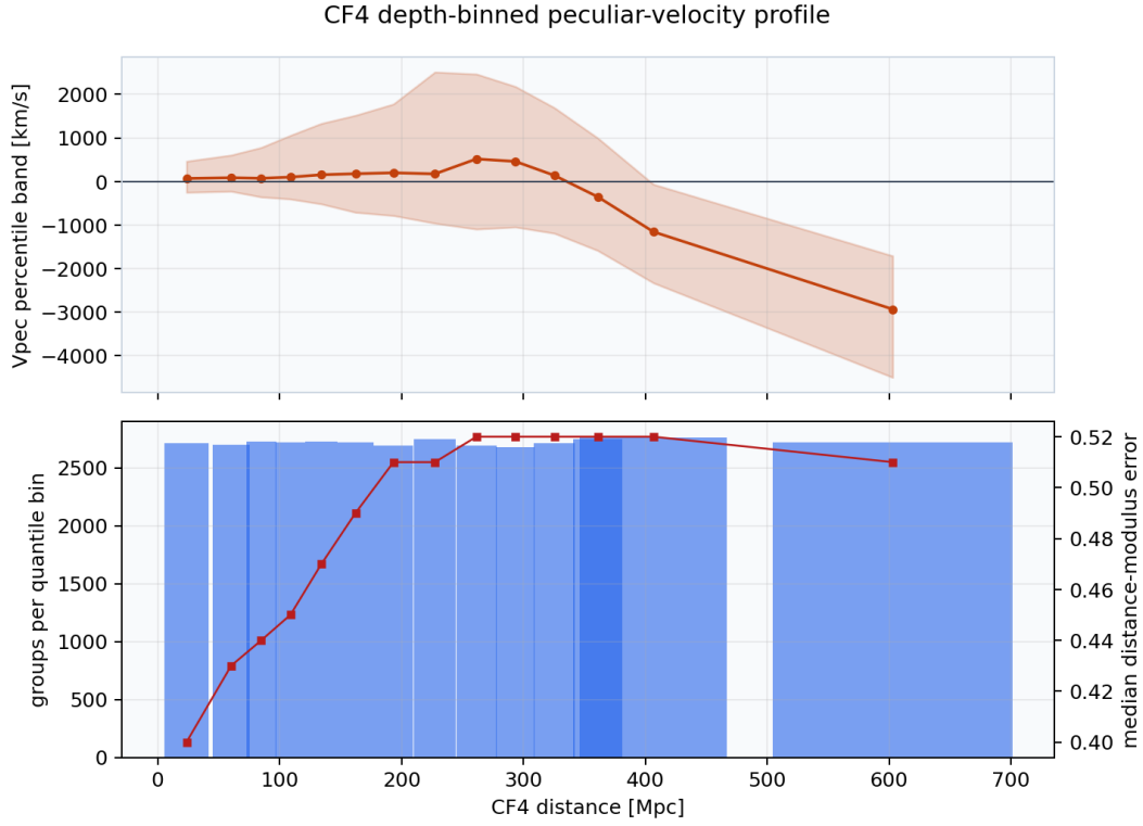
Figure 19: Cosmicflows-4 distance-binned peculiar-velocity percentile profile and group counts.
