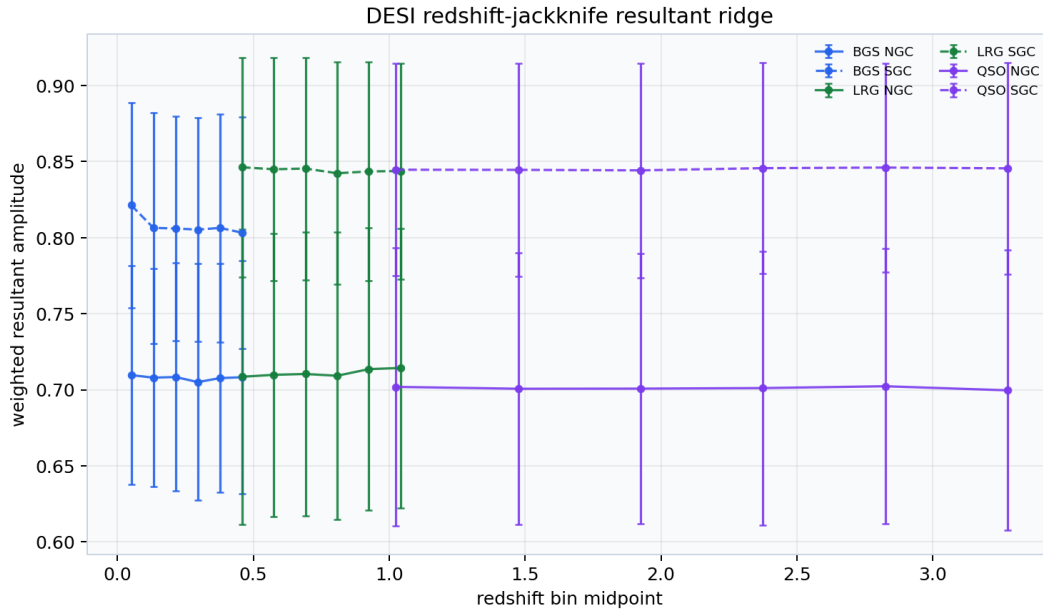
Figure 25: DESI BGS/LRG/QSO resultant amplitudes by cap and redshift bin with jackknife uncertainty.
