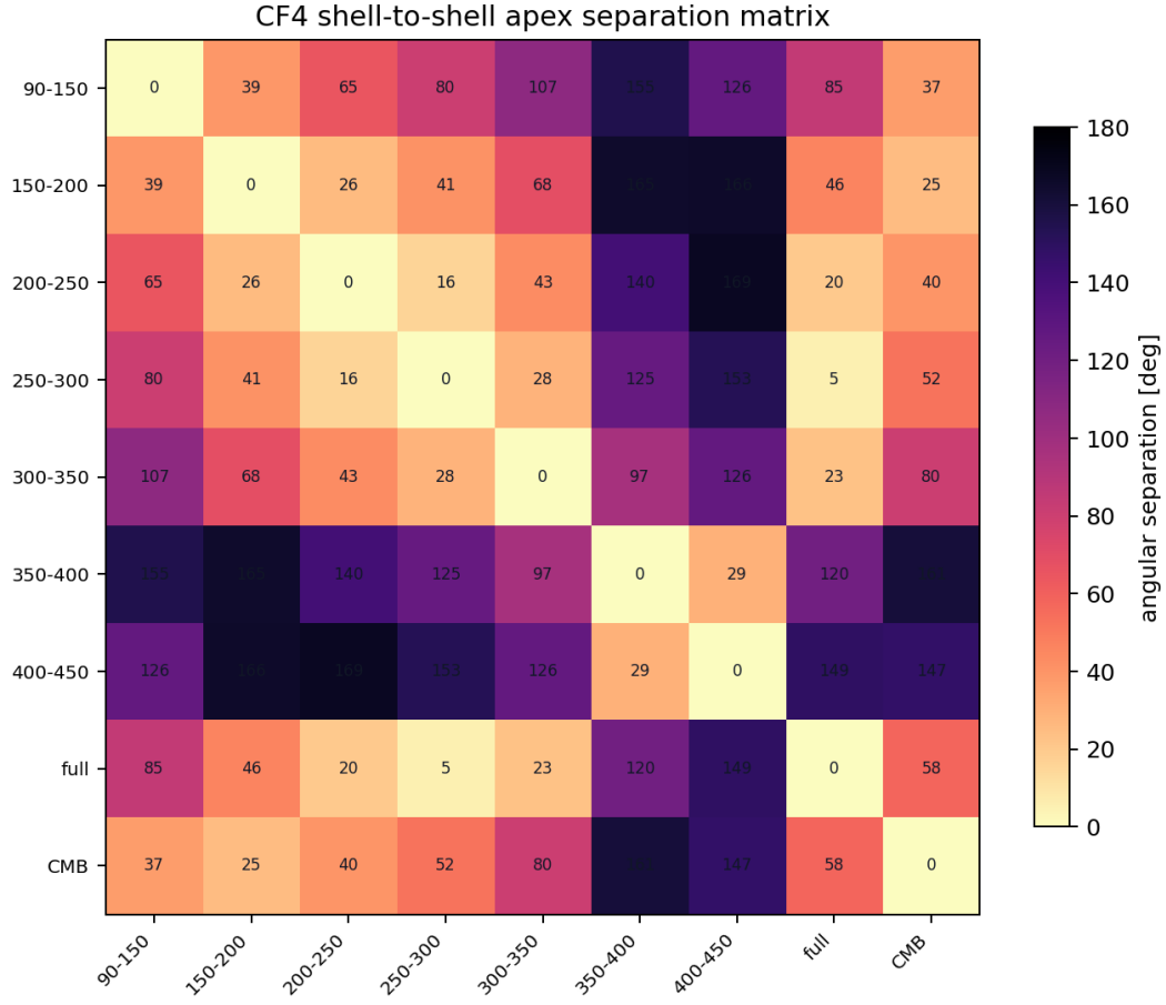
Figure 31: Pairwise angular separations among CF4++ reconstruction-functional shell apexes; no observed amplitude or global-tilt claim.
