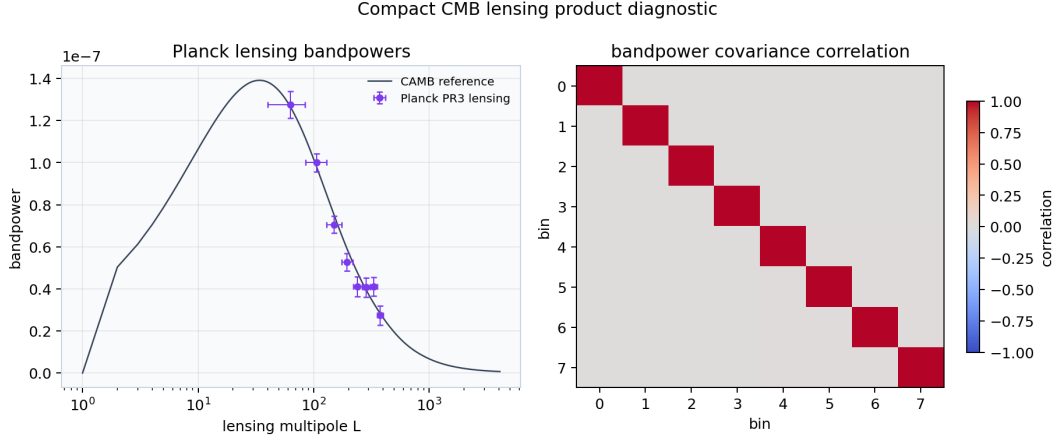
Figure 22: Planck PR3 lensing bandpowers and covariance correlation against the bundled CAMB reference.
