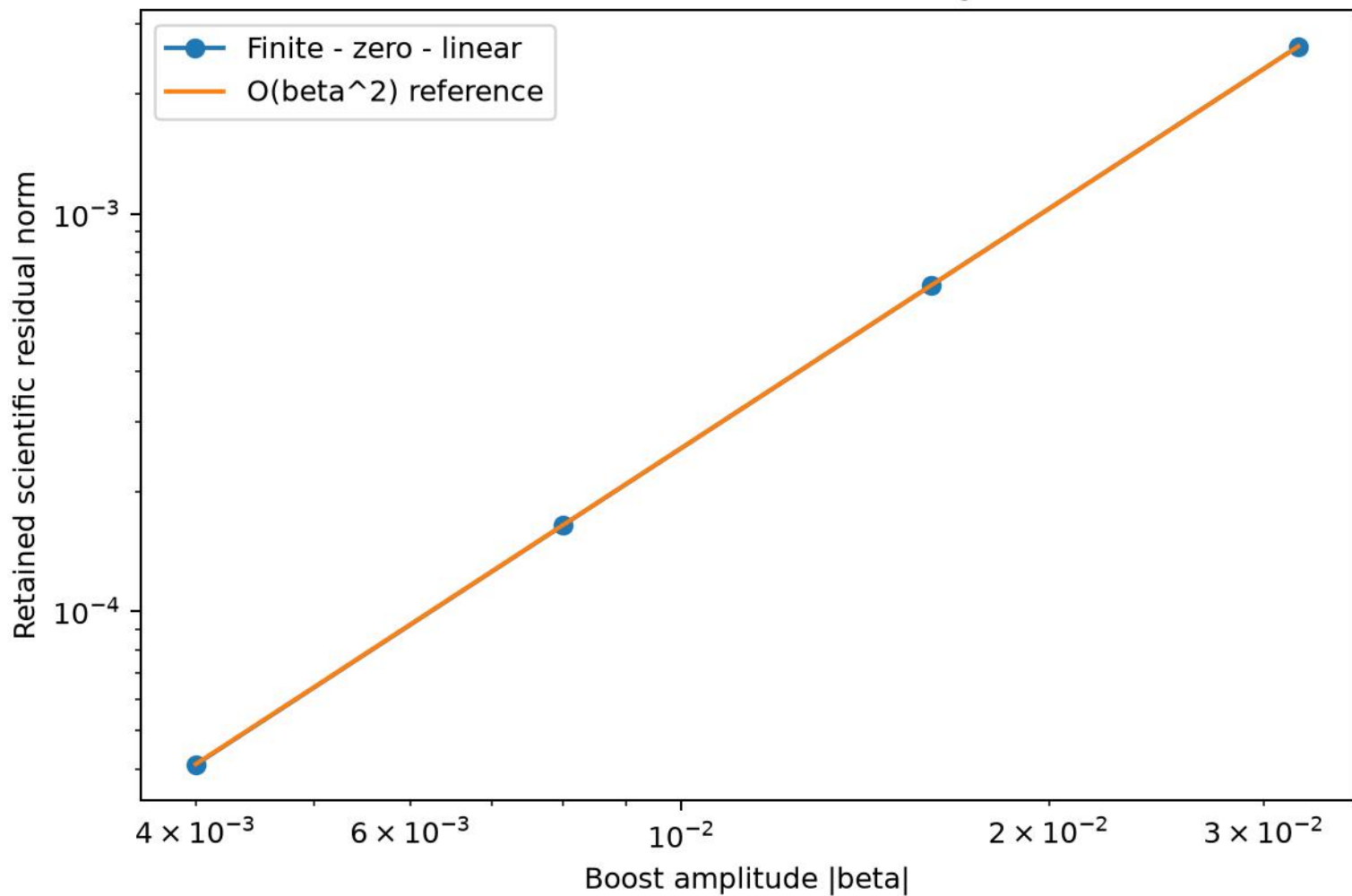
WU-011 finite-to-linear convergence
