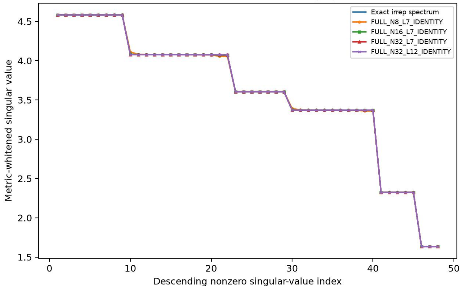
WU-011 exact and HEALPix full-sky spectra
