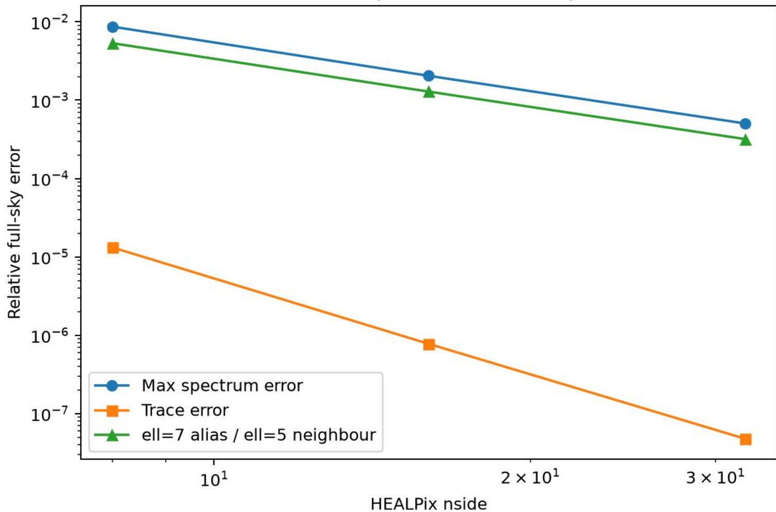
WU-011 full-sky resolution convergence
