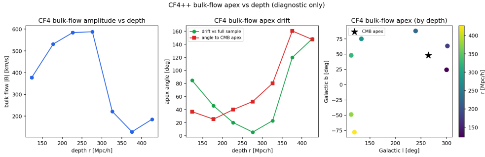
Figure 6: K4: CF4++ bulk-flow amplitude and apex drift versus depth shell. Model-independent kinematic descriptor; not a frame-violation or Bianchi claim.
