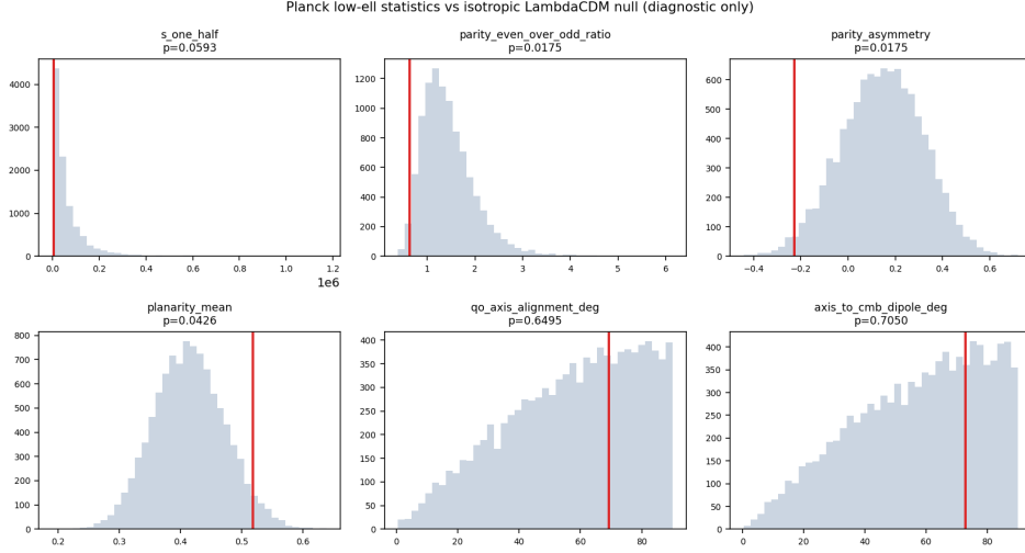
Figure 4: K1: observed low- \ell statistics of the Planck PR3 map against the isotropic \Lambda CDM null ensemble. Model-independent null-calibrated features; not evidence for any Bianchi model.
