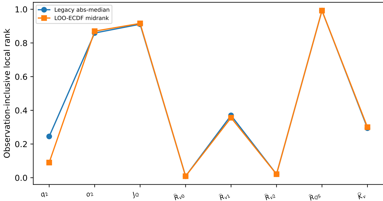
SMICA observation in the CMB-only 999 pool
