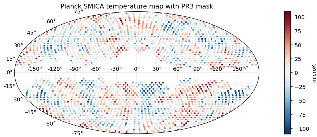
Figure 17: Planck SMICA nside16 temperature pixels displayed under the PR3 temperature mask.
