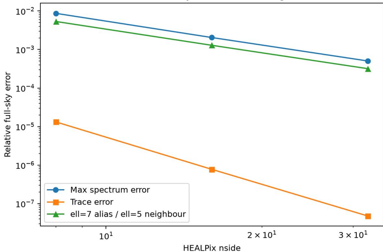
WU-011 full-sky resolution convergence
