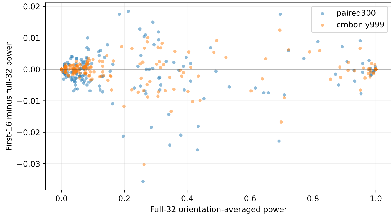
Descriptive orientation-prefix sensitivity
