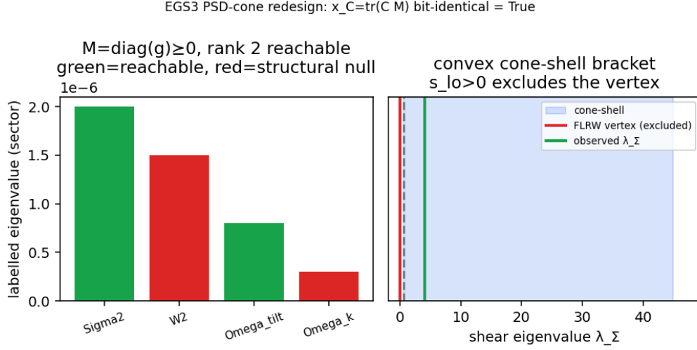
Figure 17: EGS3 PSD-cone redesign. Left: M = \text{diag}(g) \geq 0 , rank-two reachable eigen-directions (green) versus the structural null (red). Right: the convex cone-shell \{M \succeq 0 : s_{lo} < \lambda_\Sigma < s_{hi}\} excluding the FLRW vertex. Representation only, gated behind the additive upgrade; diagnostic-only.
