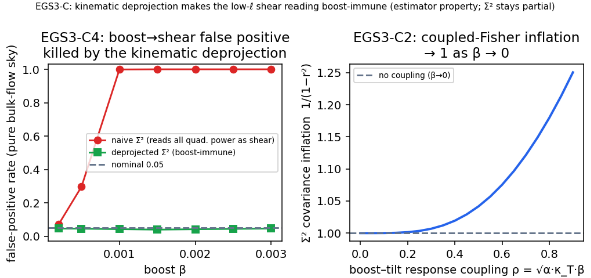
Figure 18: Axis C, kinematic deprojection of the observer-boost quadrupole. Left: on a pure-bulk-flow sky the naive \Sigma_{std}^2 false-positive rate (red) rises to nearly one as the boost \beta grows, while the deprojected \Sigma_{std}^2 (green) stays at the nominal level. Right: the coupled-Fisher \Sigma_{std}^2 covariance inflation 1/(1-r^2) versus the boost-tilt response coupling \rho = \sqrt{\alpha} \kappa_T \beta , returning to unity as \beta \rightarrow 0 . Deterministic moment-level synthetic mechanics; diagnostic-only; no map, no native low- \ell solver, no real data; \Sigma_{std}^2 stays partial.
