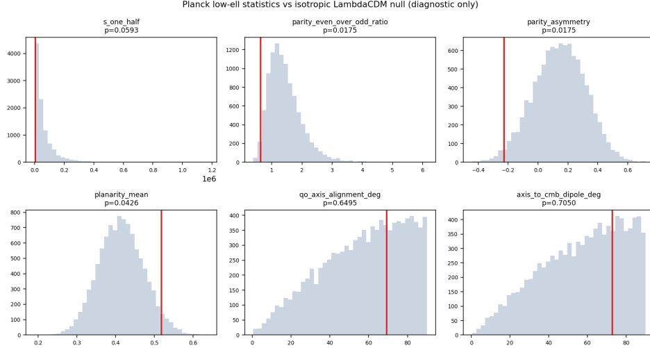
Figure 8: K1: observed low- \ell statistics of the Planck PR3 map against the isotropic \Lambda CDM null ensemble. Model-independent null-calibrated features; not evidence for any Bianchi model.
