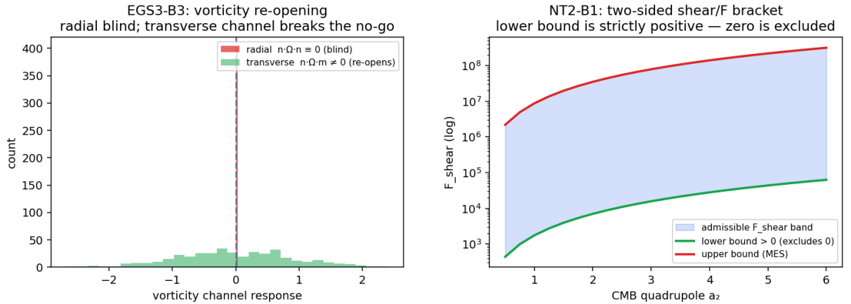
Figure 16: Axis B. Left: EGS3-B3, radial peculiar velocities are vorticity-blind ( n^a\Omega_{ab}n^b \equiv 0 ) while the transverse channel re-opens the sector. Right: NT2-B1, the two-sided shear/ F bracket; within the registered closure/H3 model the lower bound is strictly positive so the closure-defined shear-filling is excluded from zero at fixed a_2 . Diagnostic-only; synthetic.
