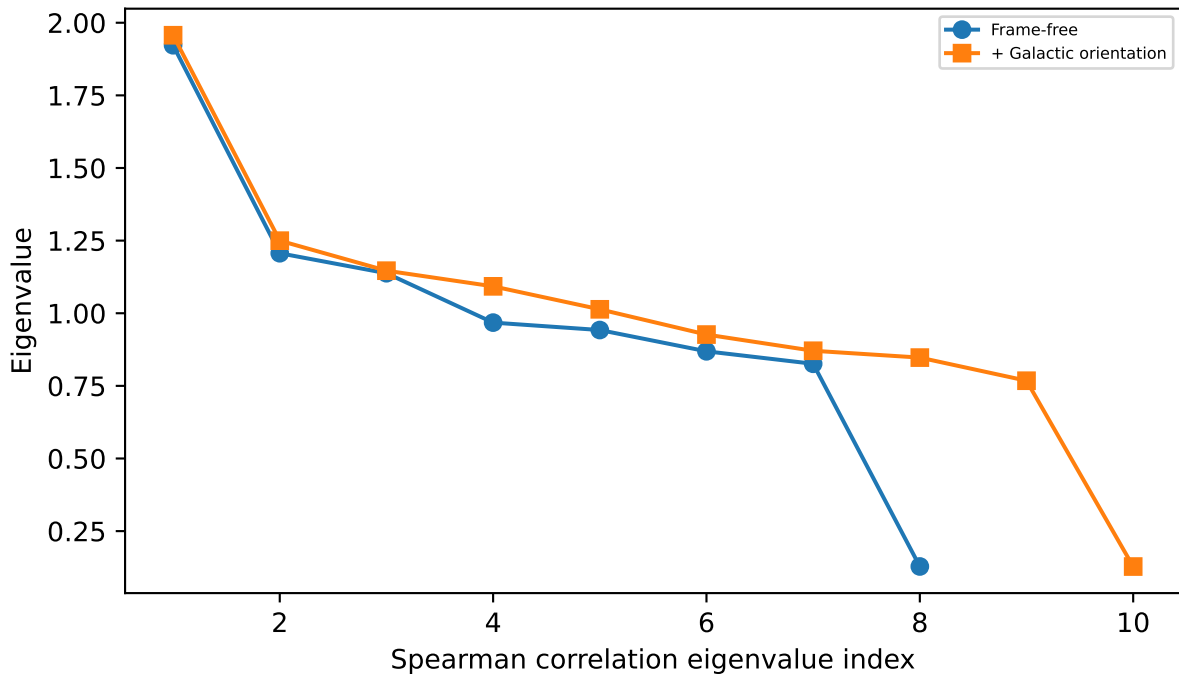
Coordinate dependence spectrum
