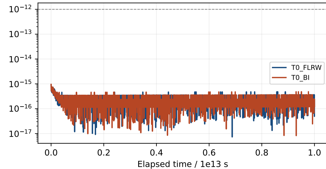
Per-step ledger residual (gate 1e-12)
