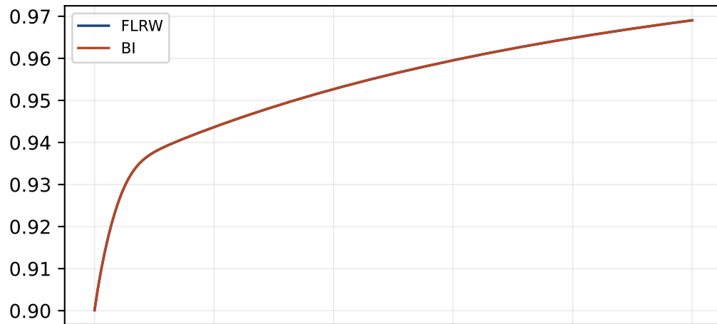
H ionized fraction
