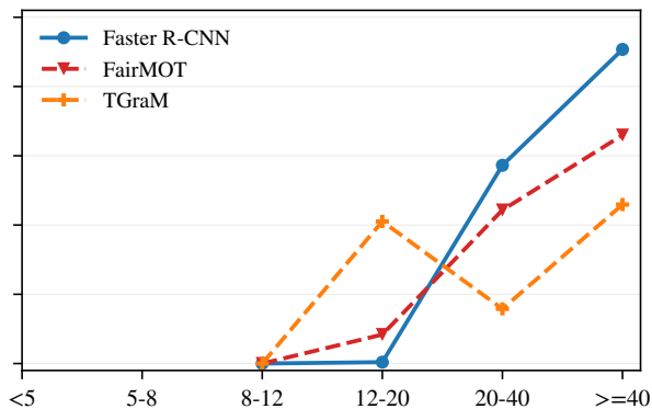
train
