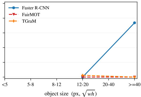
train
