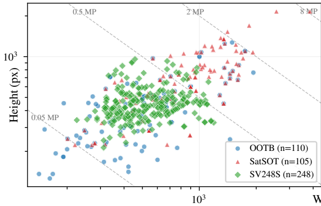
SOT benchmarks
