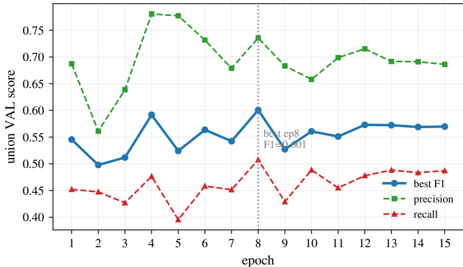
HiEUM car-union retrain — per-epoch VAL
