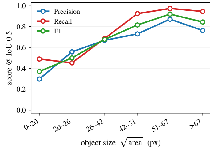
Faster R-CNN
