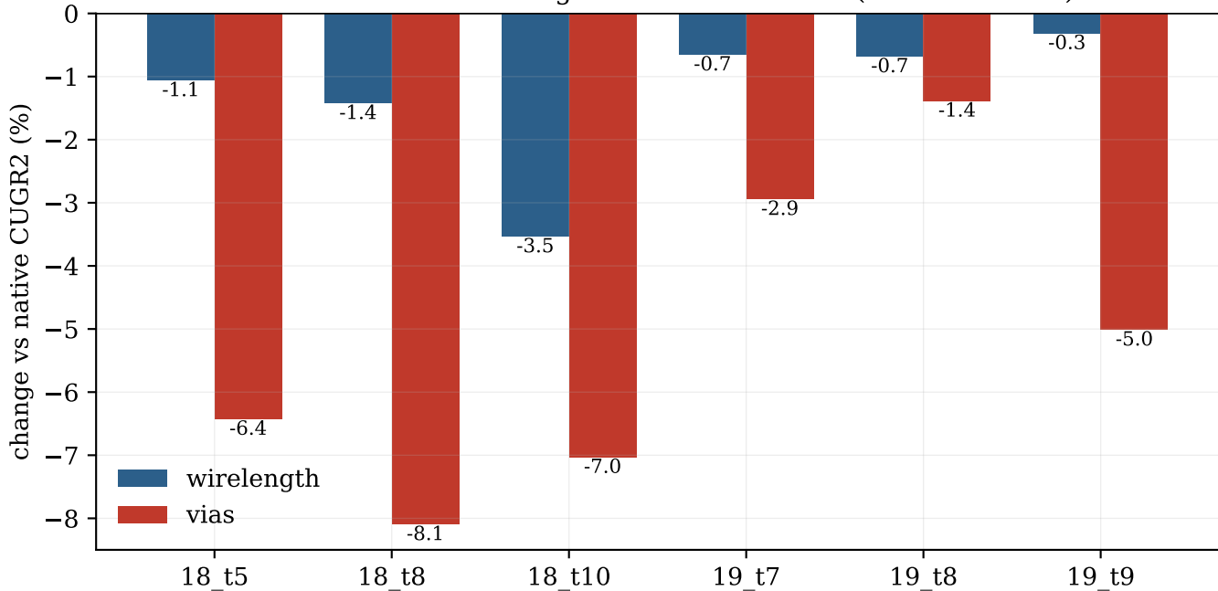
Ours vs native: wirelength and via reduction (lower is better)
