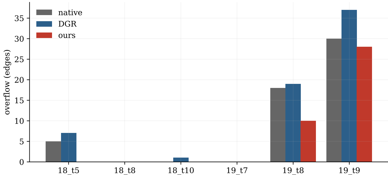
Overflow: native vs DGR vs ours (CUGR2-measured)
