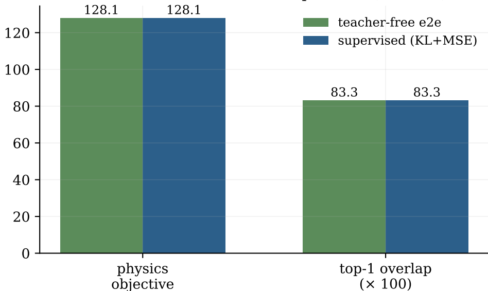
Teacher-free e2e matches supervised (held-out)
