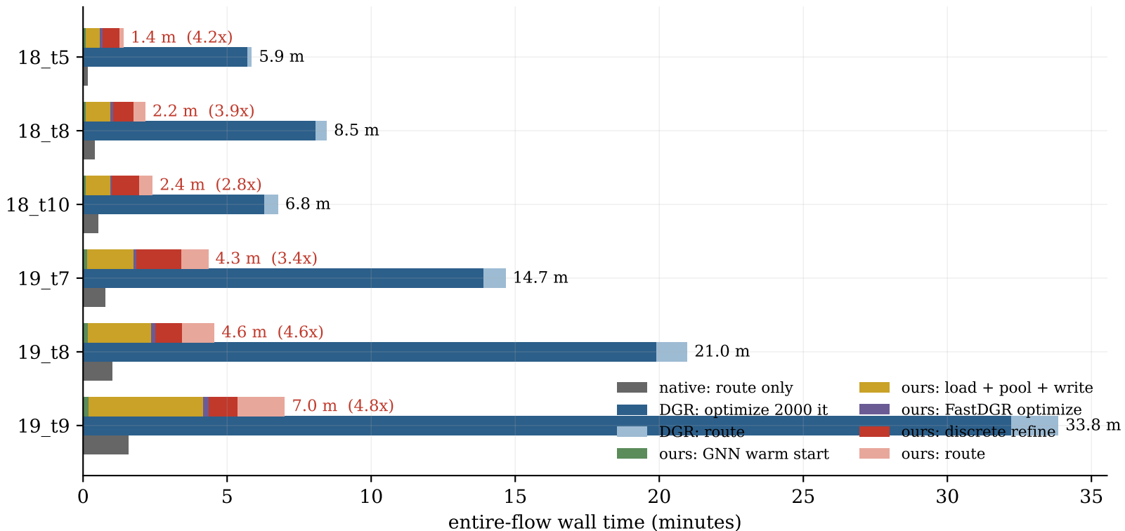
Entire flow (all overhead + CUGR2 route): native vs DGR vs ours
