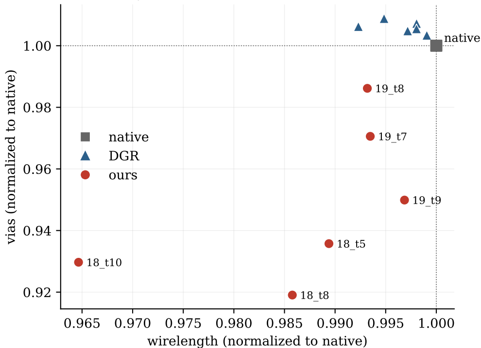
Quality relative to native (lower-left is better)
