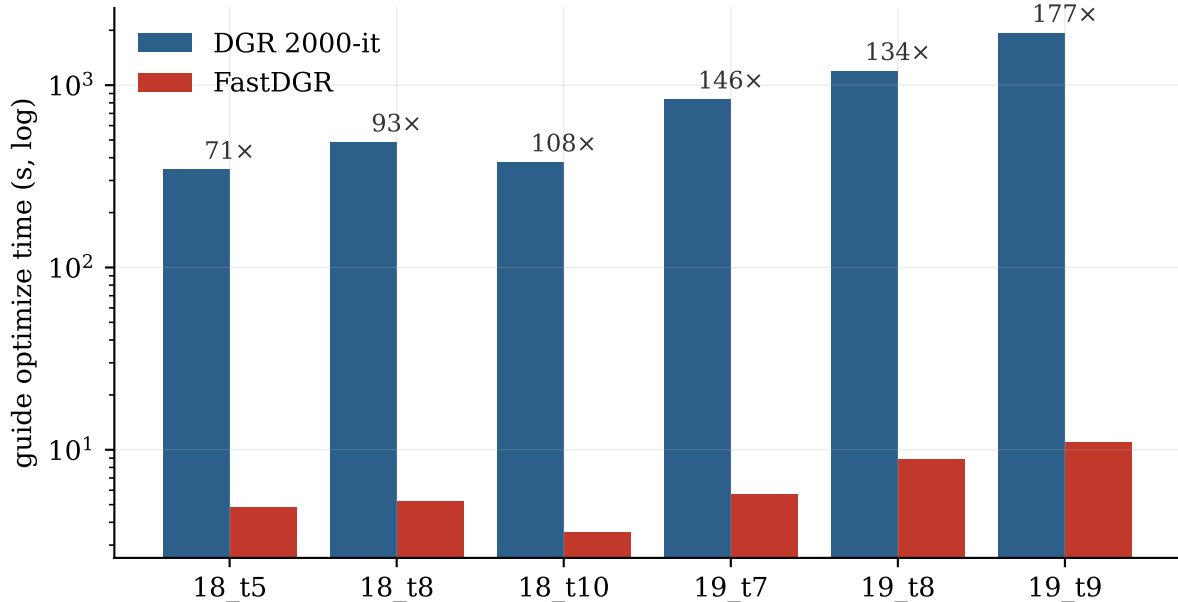
Guide-generation time: DGR vs FastDGR
