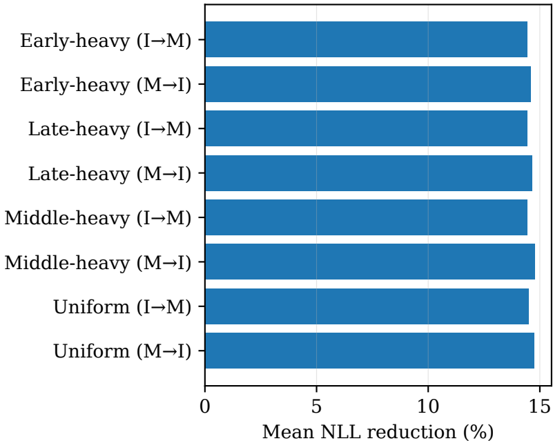
Training-derived calibration
